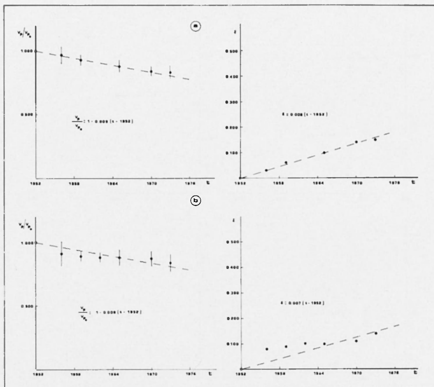
Fig. 4 - Maina di Sauris dam. Representation of \nu_r and \varepsilon values versus time (in years), with indication of most probable trends.
