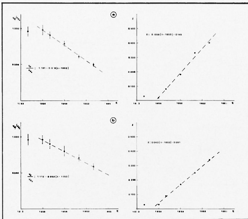
Fig. 6 - Vajont dam. Representation of \nu_p and \epsilon values versus time (in years), with indication of most probable trends.
