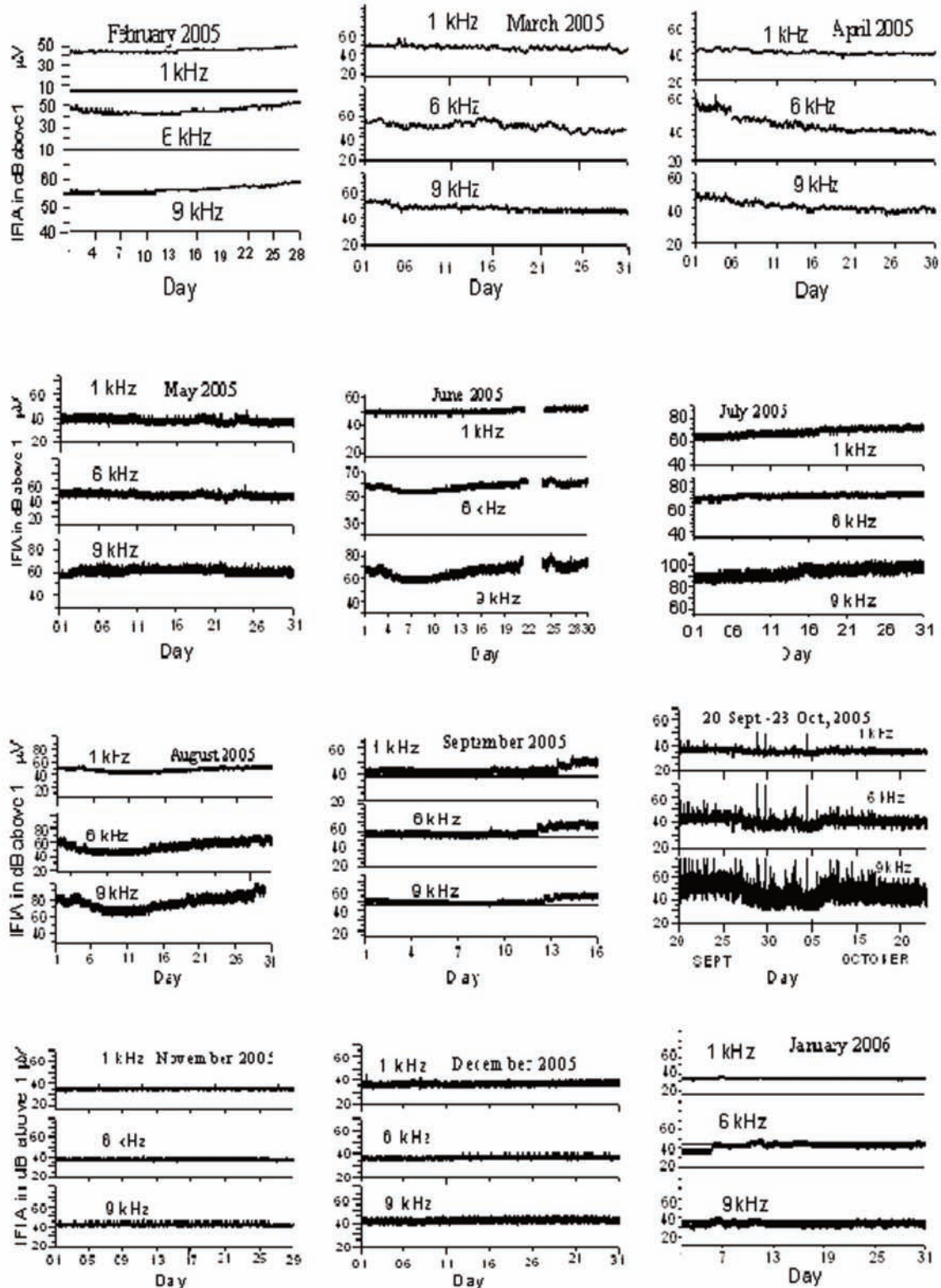
Figure 3. Time series records of the IFIA at 1 kHz, 6 kHz and 9 kHz for the months of February 2005 to January 2006.
