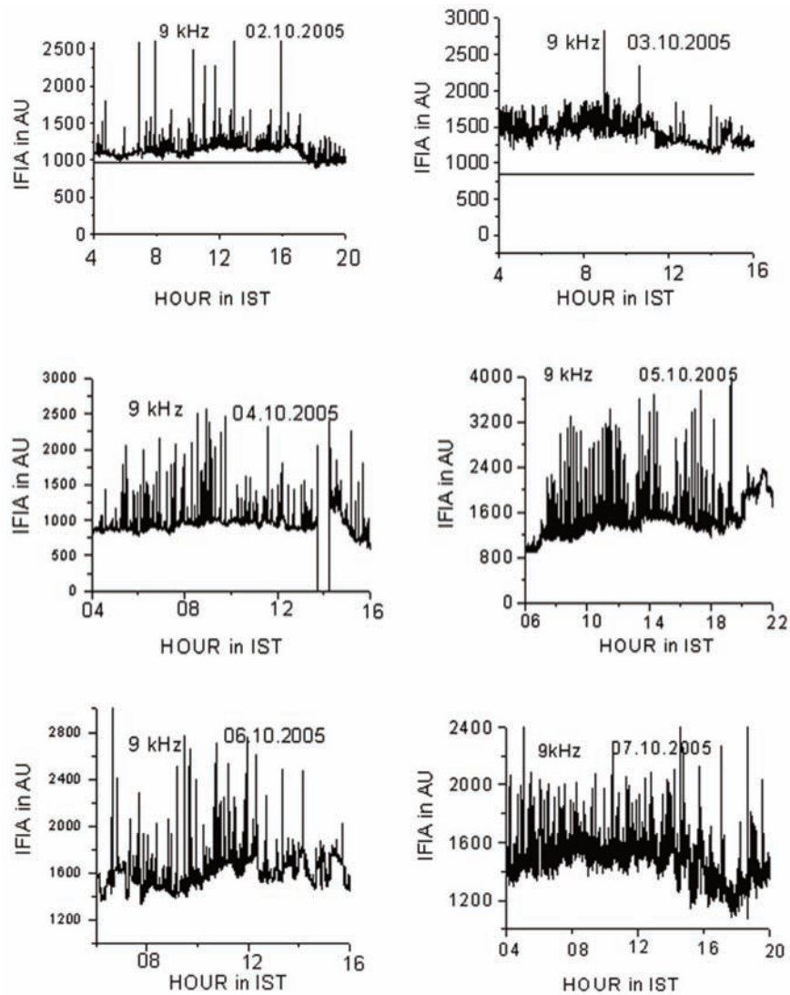
Figure 19. Variations of the IFIA at 9 kHz recorded from October 2–7, 2005, at Mirik (latitude, 26.9^{\circ} N; longitude, 88.17^{\circ} E).
