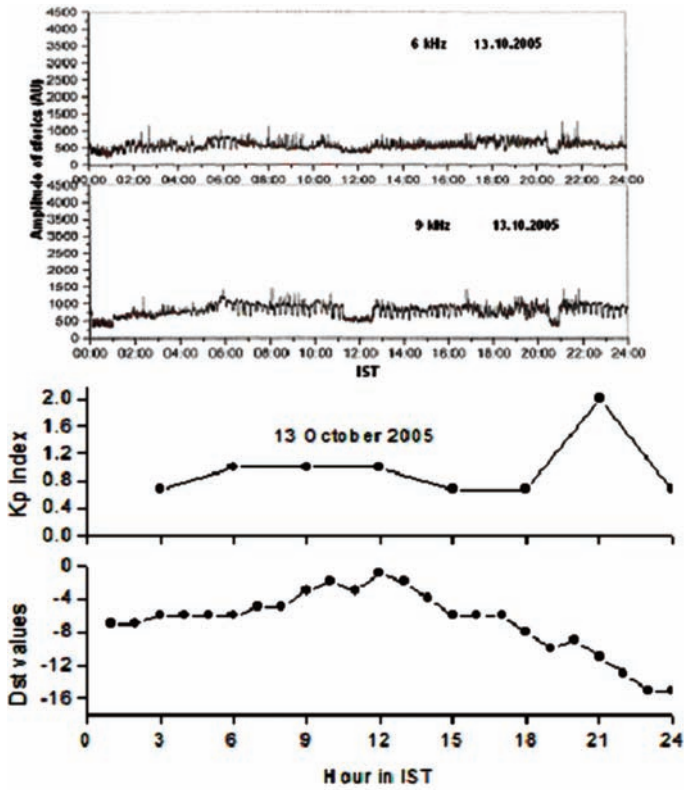
Figure 15. Diurnal variations of the IFIA at 6 kHz and 9 kHz, and of the Kp index and Dst, for Agartala on October 13, 2005.
