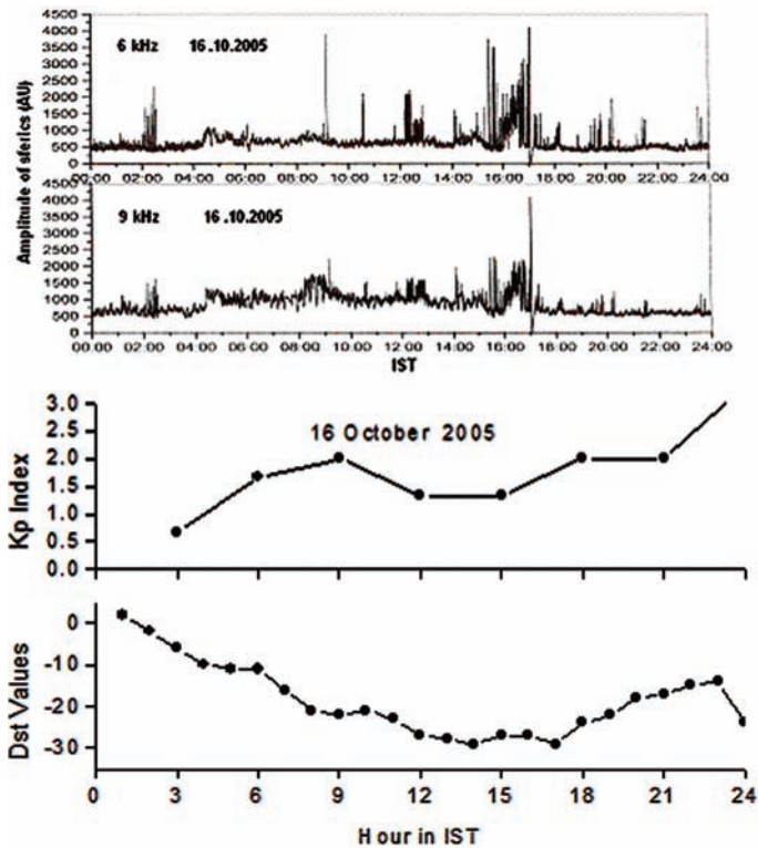
Figure 16. Diurnal variations of the IFIA at 6 kHz and 9 kHz, and of the Kp index and Dst, for Agartala on October 16, 2005.
