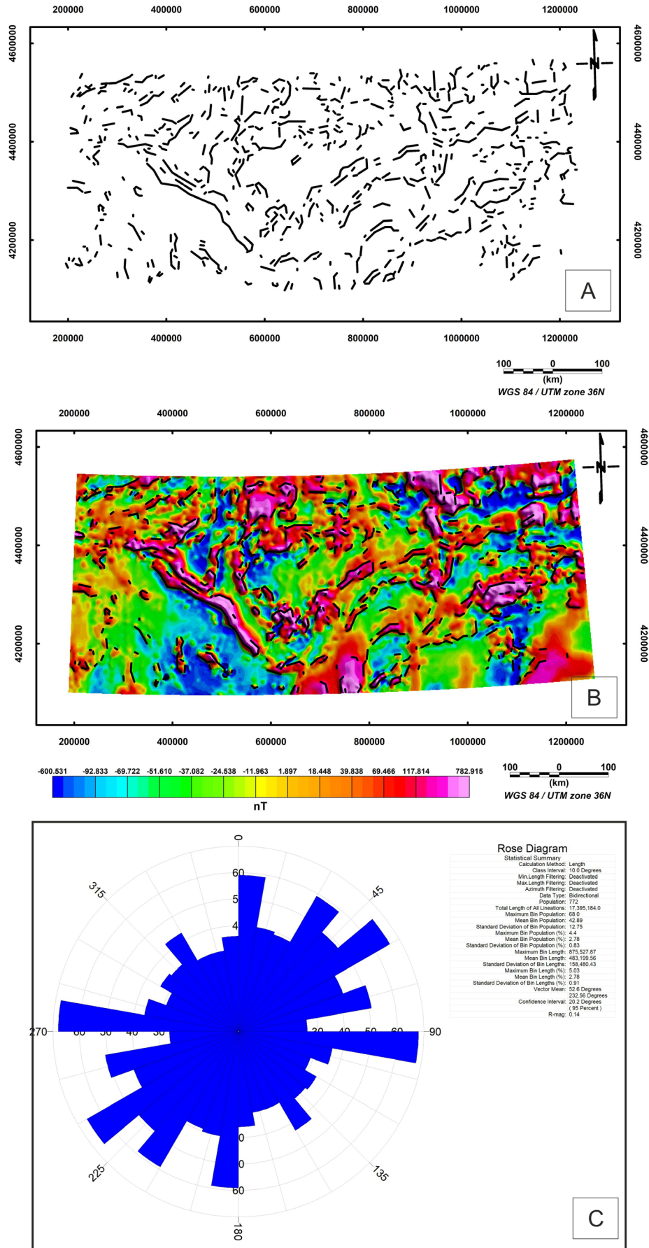
Figure 10. (a) Magnetic lineament map of the study area. (b) Superimposed map of the RTP magnetic anomaly and lineament map. (c) Rose diagram of the study area.
