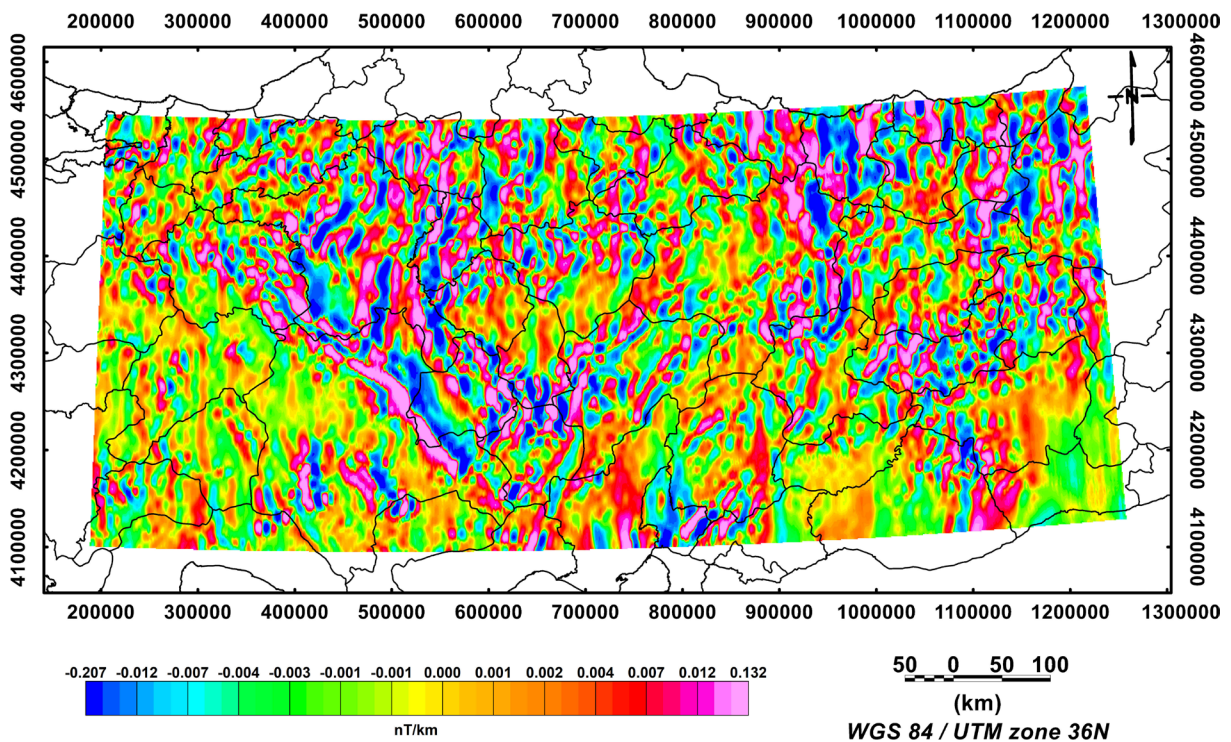
Figure 5. THG map of RTP data (Black continuous lines on the map indicate the city boundaries of the study area).
