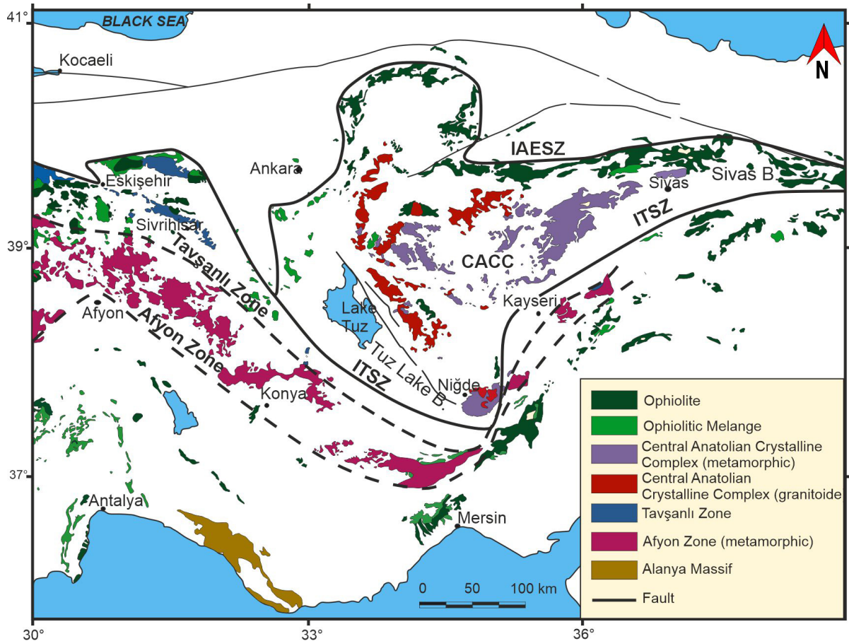
Figure 2. Geological map of the study area (Modified after MTA, 2002; van Hinsbergen et al., 2016; Pourteau et al., 2010; Çrtk et al., 2024).
