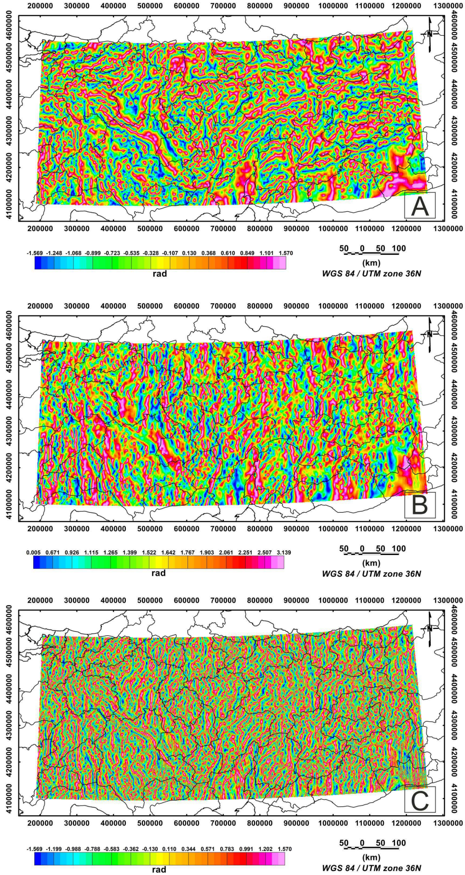
Figure 6. (a) TA map of RTP data. (b) TM map of RTP data. (c) TAHG map of RTP data (Black continuous lines on the map indicate the city boundaries of the study area).
