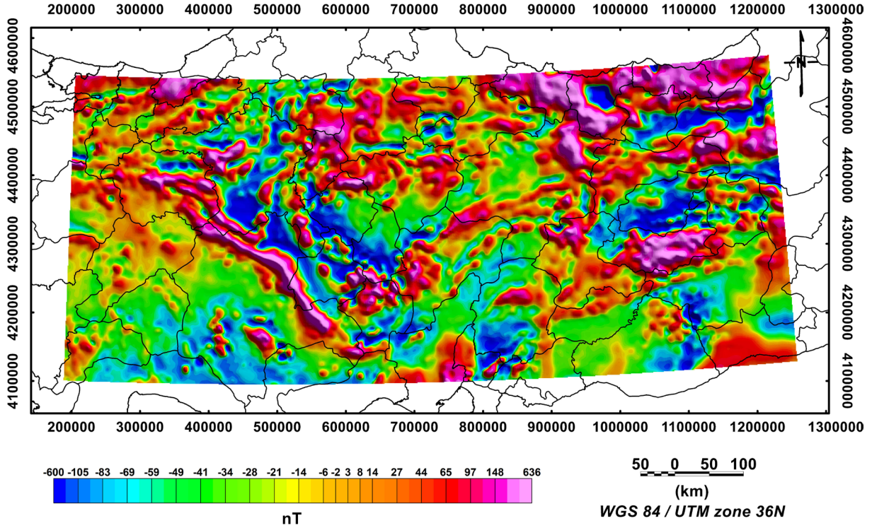
Figure 3. Total magnetic anomaly map (Black continuous lines on the map indicate the city boundaries of the study area).
