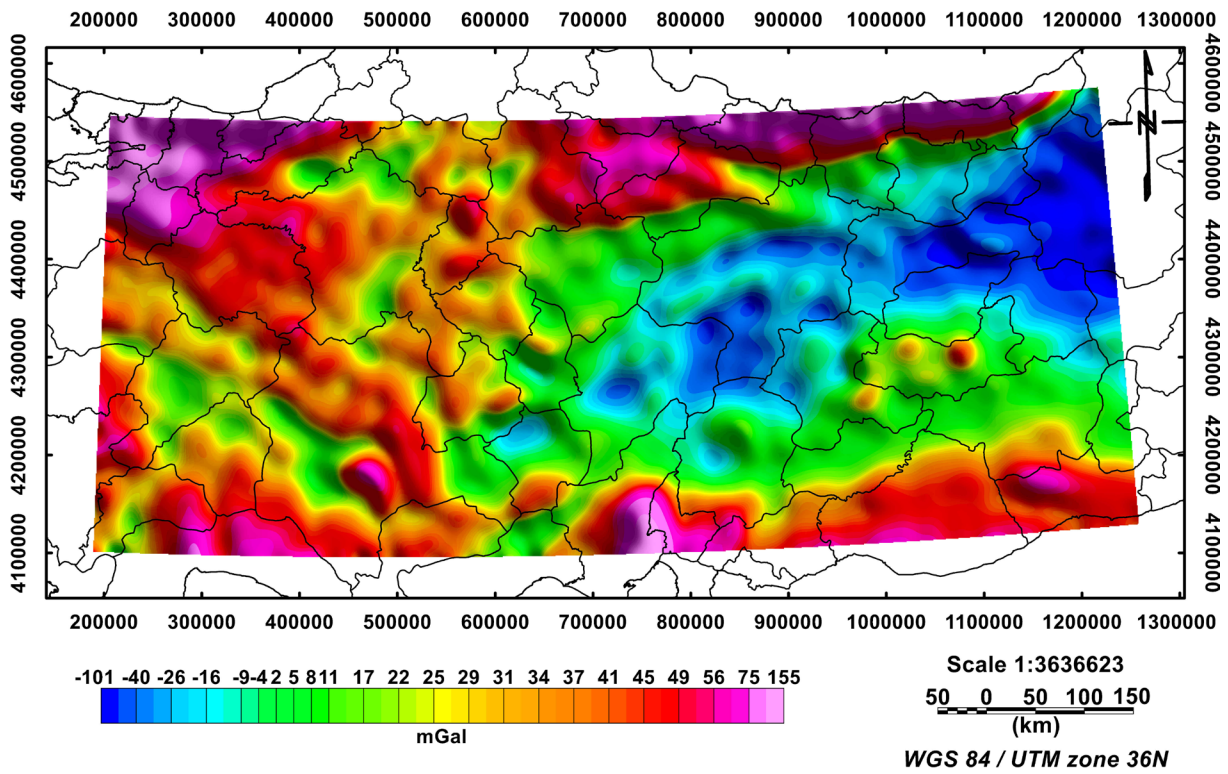
Figure 7. Bouguer gravity data (Black continuous lines on the map indicate the city boundaries of the study area).
