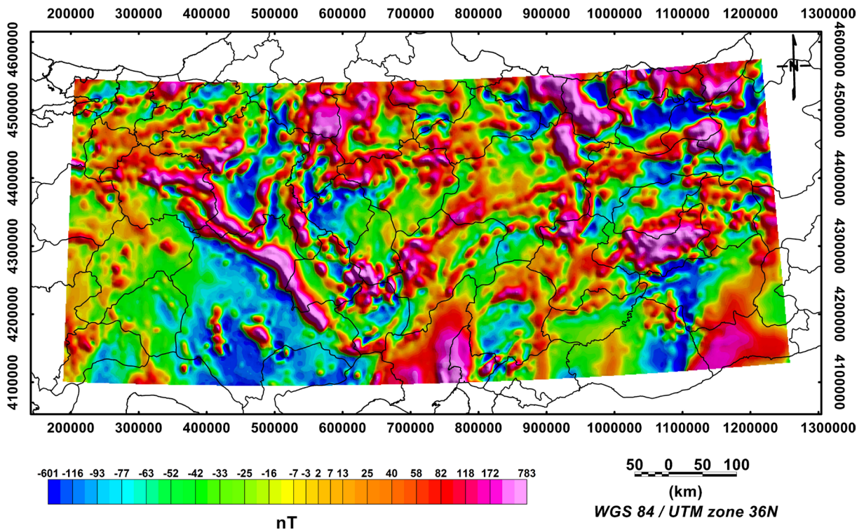
Figure 4. RTP magnetic anomaly map (Black continuous lines on the map indicate the city boundaries of the study area).
