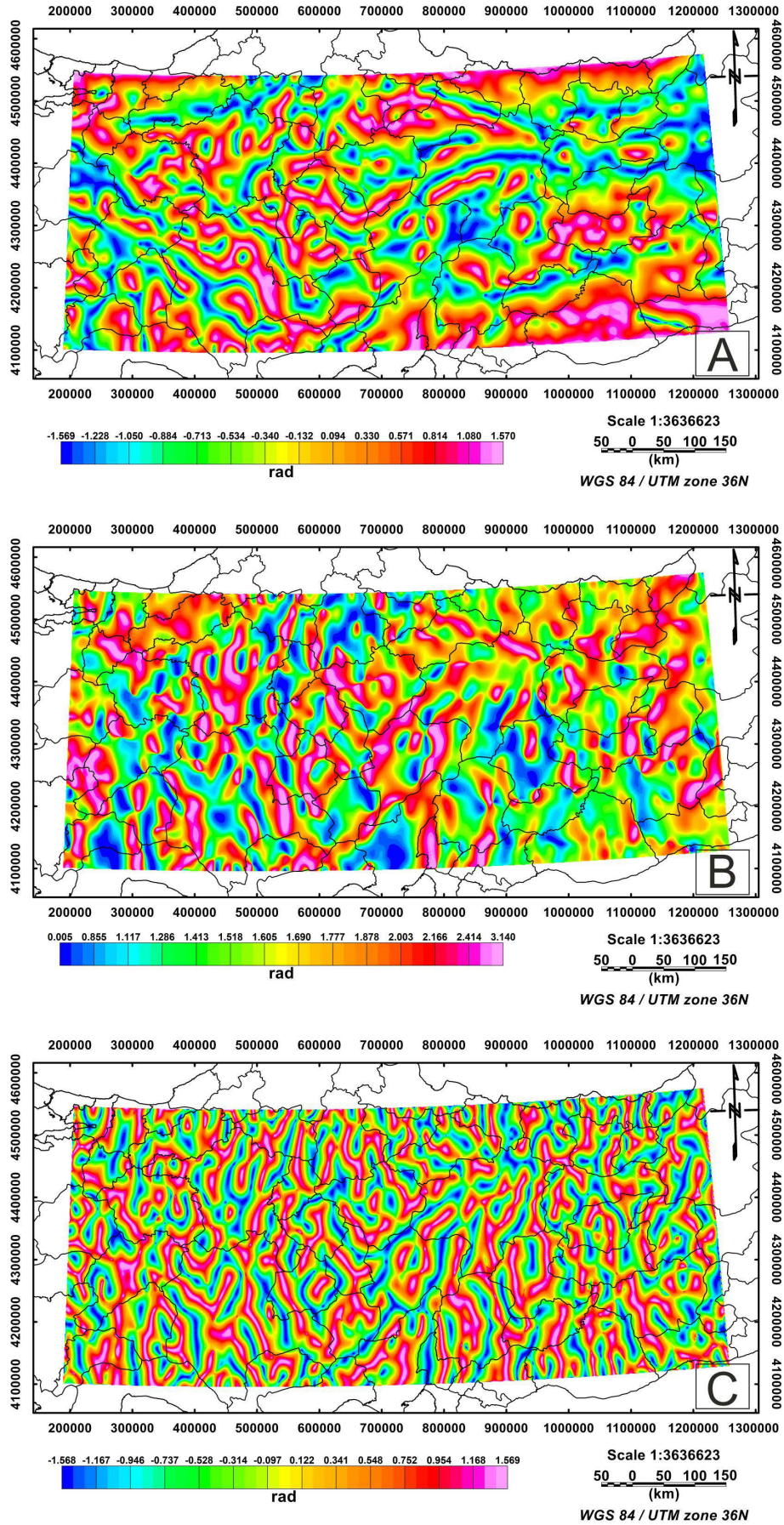
Figure 9. (a) TA map of Bouguer gravity data. (b) TM map of Bouguer gravity data. (c) TAHG map of Bouguer gravity data (Black continuous lines on the map indicate the city boundaries of the study area).
