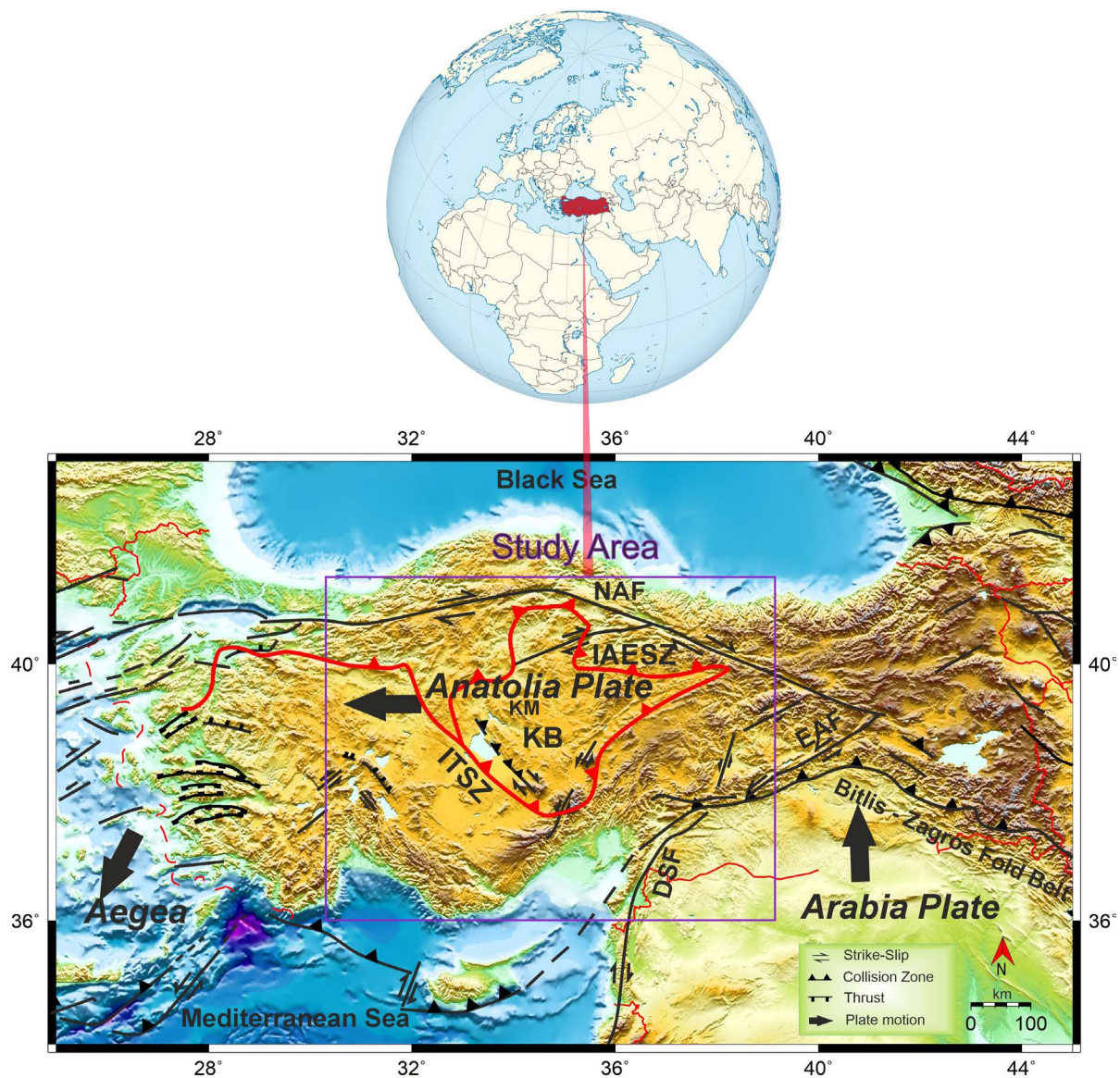
Figure 1. Tectonic map of Turkey and the surrounding areas (Modified from řarođlu et al., 1992; Bozkurt, 2001; Taymaz et al., 2007; and Emre et al., 2013). Abbreviations: EAF: East Anatolian Fault, NAF: North Anatolian Fault, DSF: Dead Sea Fault, KM: Kırřehir Massif, KB: Kırřehir Block, IAESZ: İzmir-Ankara-Erzincan Suture Zone, ITSZ: Inner Tauride Suture Zone. The base map was created using General Mapping Tools (GMT) (Wessel et al., 2013). The study area is shown with a purple square.
