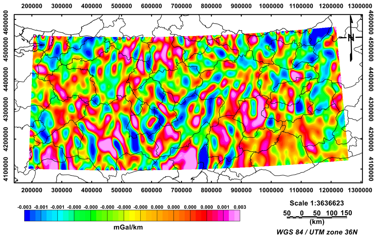
Figure 8. THG map of Bouguer gravity data (Black continuous lines on the map indicate the city boundaries of the study area).
