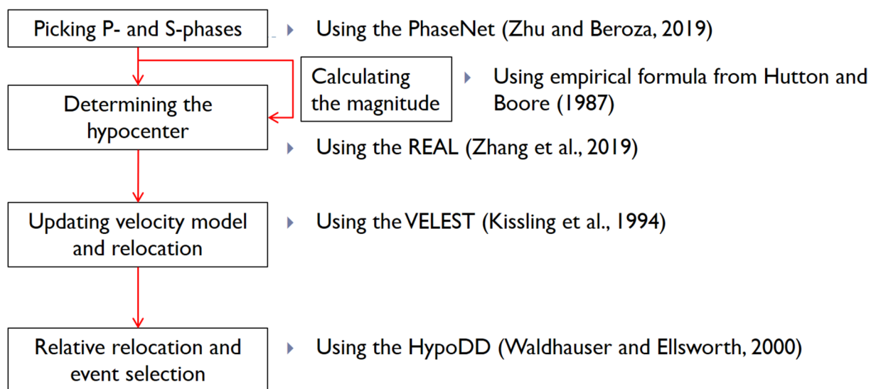
Figure 4. The workflow we followed to determine the aftershock catalog for the 2006 Yogyakarta M_W \sim 6.4 earthquake.
