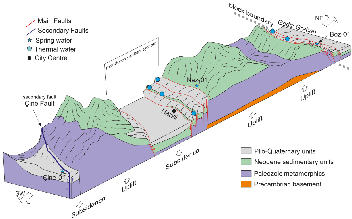
Figure 6. Geological and tectonic illustration on vicinity of the spring water regions. Orientation and the location of the cross section is shown at Fig. 1. Note that, spring waters are located on different faults. Naz-01 is located on Menderes fault, Çine-01 is located on a secondary fault and Boz-01 is located on Gediz fault which is within adjacent block. Modified and interpreted based on İnan et al. (2010).
