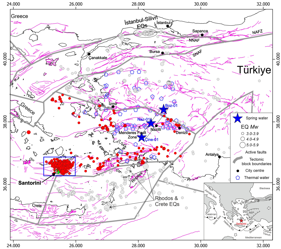
Figure 1. Location of the study area and tectonic setting. Map is constructed with longitude coordinate system, elevations are on wgs84 format. The inset map shows current tectonic setting of Aegean Sea and surroundings. Studied are Aegean Extensional Province (AEP) is indicated. Main map displays the active fault map of the Western Anatolia, Aegean Sea. Location of the spring waters (Naz-01, Çine-01 and Boz-01) are indicated as blue star. Black rectangle is the area of cross-section shown in Fig. 6. Magenta lines represent the active faults (Emre et al., 2012; Ganas et al., 2013). Plotted EQs cover the time between May 2023 to July 2025. Dark gray thick lines show the previously published microplate boundaries that is edited from Nyst and Thatcher (2004) and Reilinger et al. (2006). Santorini island is highlighted in green color. Light blue pentagons represent the thermal water sites around the region. MFZ: Menderes Fault Zone, NAFZ: North Anatolian Fault Zone, NNAF: Northern branch of North Anatolian Fault, SNAF: Southern branch of North Anatolian Fault Zone. All earthquakes ( \geq 3 ) are plotted in red color (in-block EQs) and in gray color (out-block EQs) circles; diameters are scaled to earthquake magnitude ( http://www.koeri.boun.edu.tr/sismo/zeqdb/ ).
