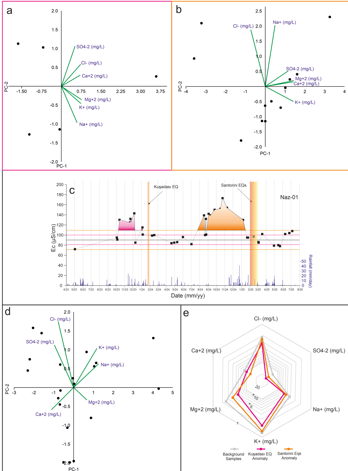
Figure 5. PCA analysis on IC results of Naz-01 spring. (a-b) Distribution and correlation factors of each ion of the anomaly before the Kuşadası EQ (Oct 2023-Dec 2023) and Santorini events (Aug 2024-Jan 2025) respectively displaying two distinct clusters of ions loading factors. (c) EC distribution of Naz-01. (d) Distribution of ions within the background samples showing dispense correlation. (e) Radar diagram of the IC averages of the background samples and samples of anomalous periods showing the differentiation of the clusters for different periods. Note that the concentrations increase from the periphery to the center.
