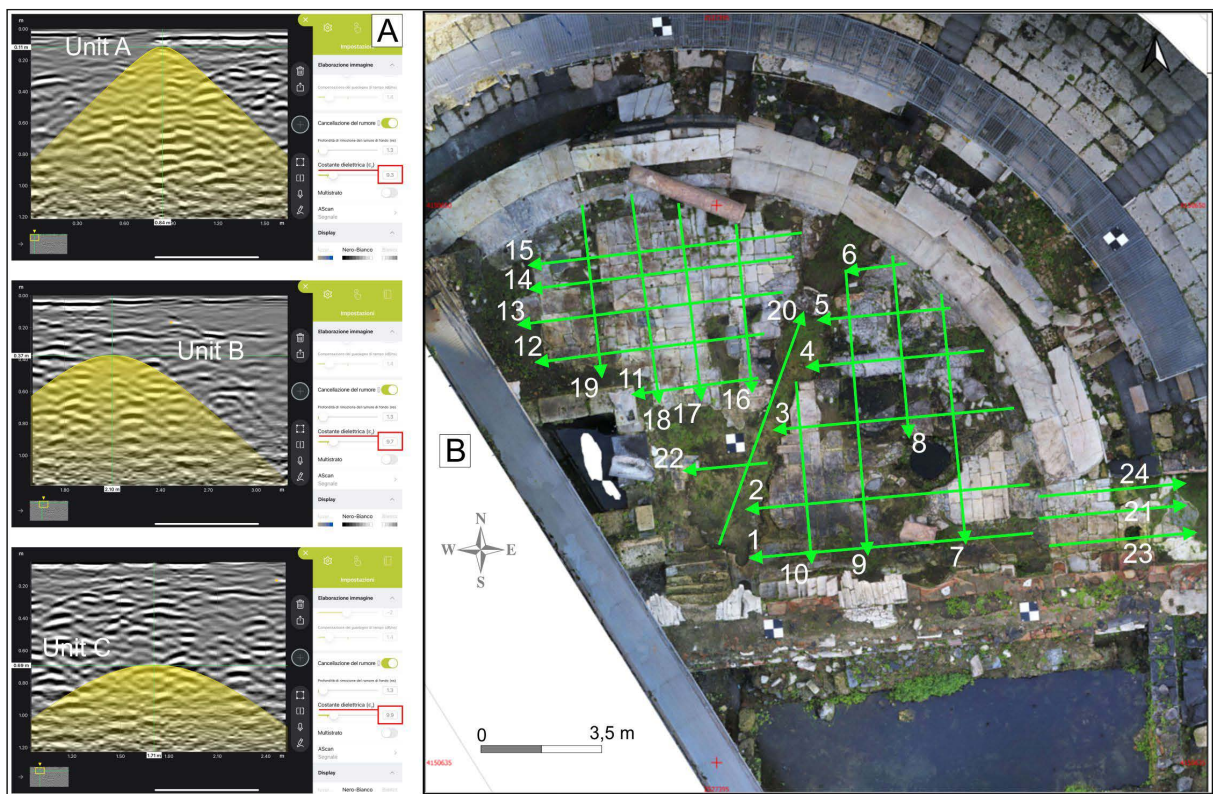
Figure 6. (a) Hyperbola fitting procedure adopted to retrieve dielectric constants for the identified electromagnetic units A, B, and C. (b) Grid of profiles acquired through georadar survey.
