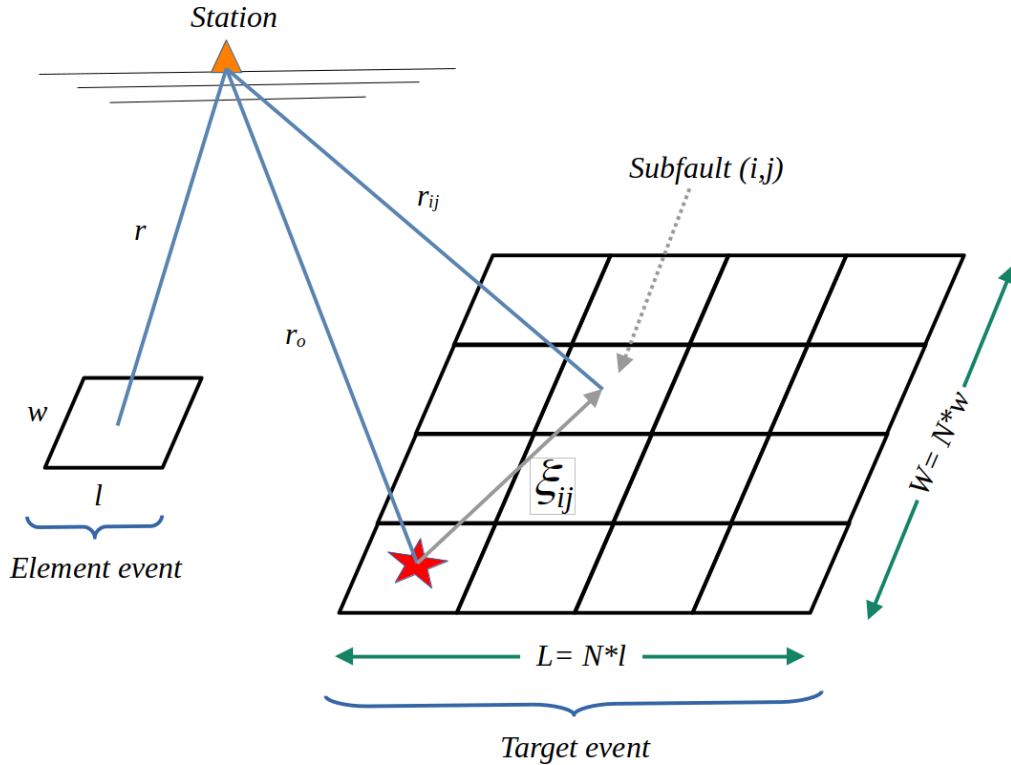
Figure 6. Schematic representation of the empirical Green's function method by Irikura (1986).
