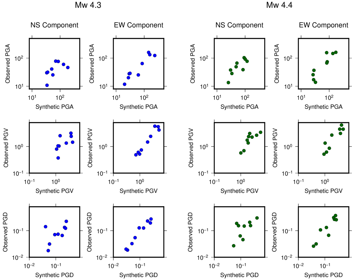
Figure 10. Comparison between observed vs synthetic peak ground displacement, velocity, and acceleration values for the Mw 4.3 (blue circles) and Mw 4.4 (green circles) events.
