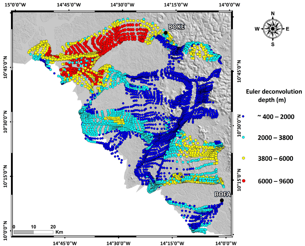
Figure 9. Euler deconvolution solutions showing the estimated depths of the magnetic sources.
