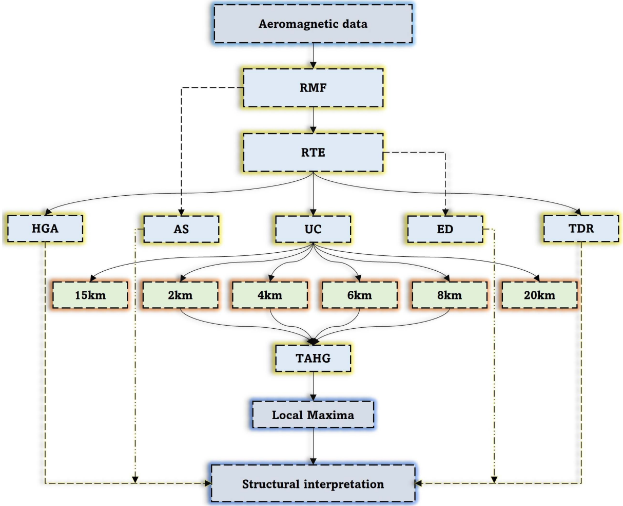
Figure 2. Processing workflow of the magnetic data illustrating the methodology adopted to accomplish the study objectives.
