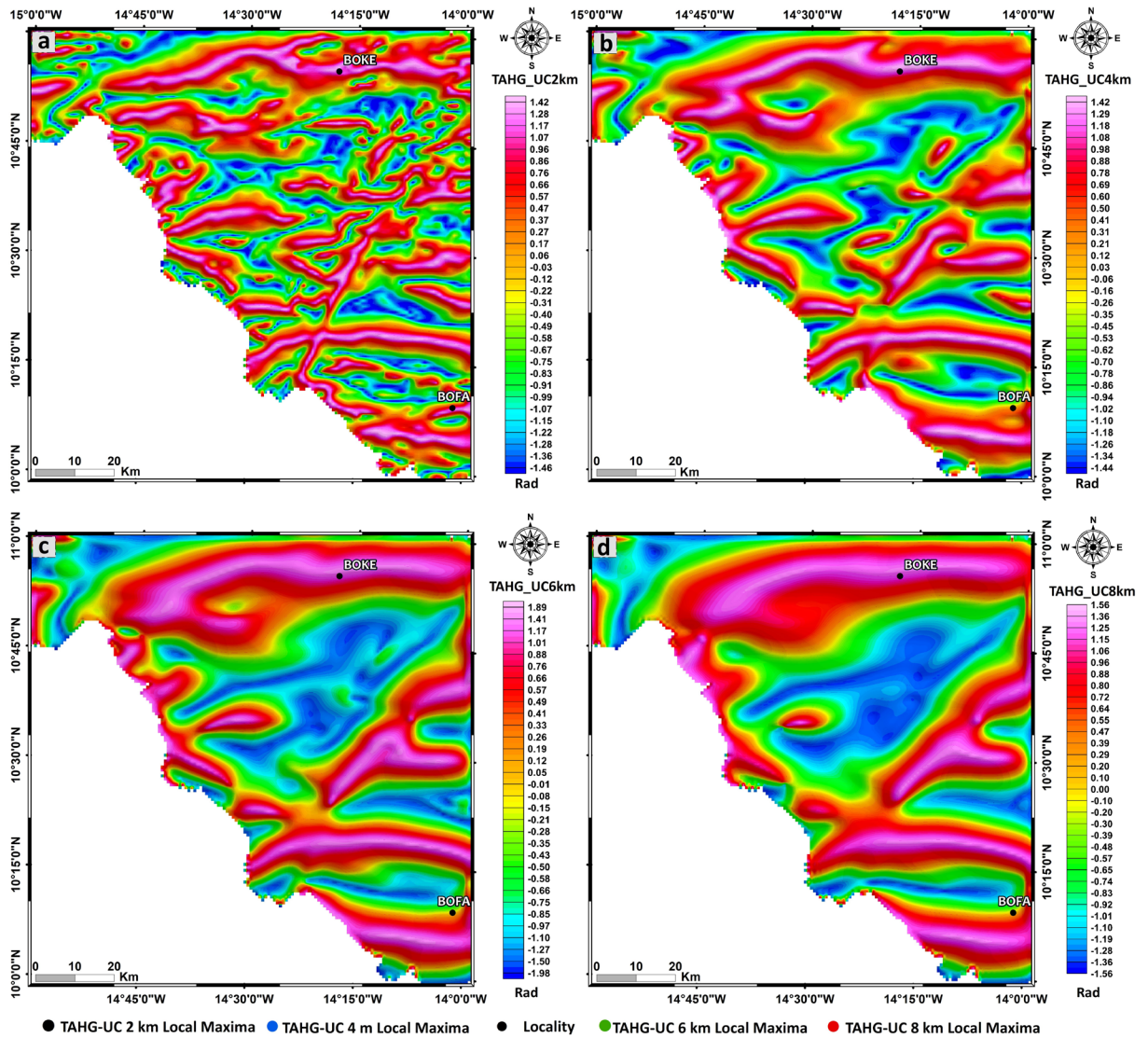
Figure 7. Tilt angle of the horizontal gradient (TAHG) computed on the upward-continued fields at 2 km (a), 4 km (b), 6 km (c) and 8 km (d).
