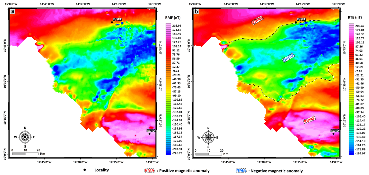
Figure 3. Residual magnetic field of the study area (a) and its reduction-to-the-equator (RTE) transform (b).
