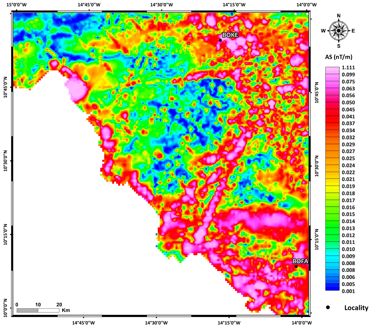
Figure 5. Analytic signal amplitude of the magnetic field of the study area.
