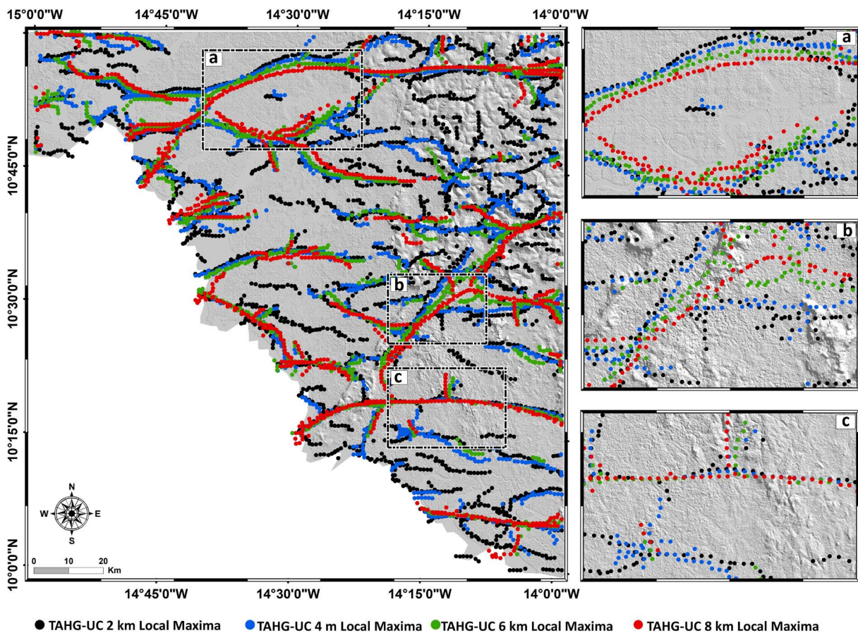
Figure 8. Local maxima map of the TAHG derived from four upward-continuation levels (black: 2 km; blue: 4 km; green: 6 km; red: 8 km).
