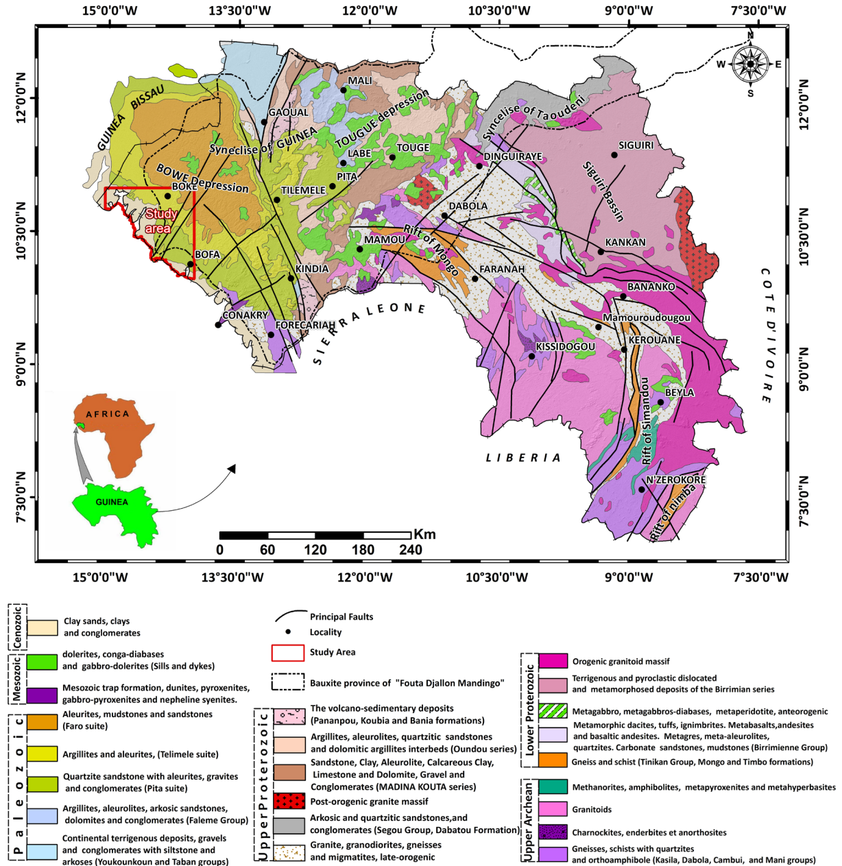
Figure 1. Geological Map of Guinea Showing Major Lithological Units and Structural Features with the Location of the Study Area (Mamedov et al., 2010b; Sangaré et al., 2024).
