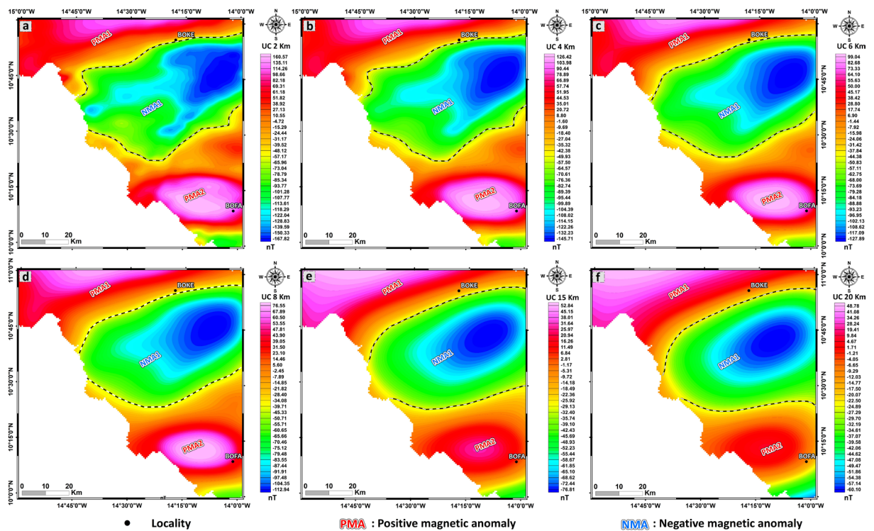
Figure 4. Upward continuation of the RTE field to 2 km (a), 4 km (b), 6 km (c) and 8 km (d), 15 km (e) and 20 km (f).
