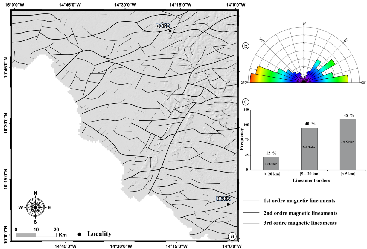
Figure 10. (a) Synthetic structural map of the study area. (b) Rose diagram of lineament orientations. (c) Frequency distribution of the three lineament orders.
