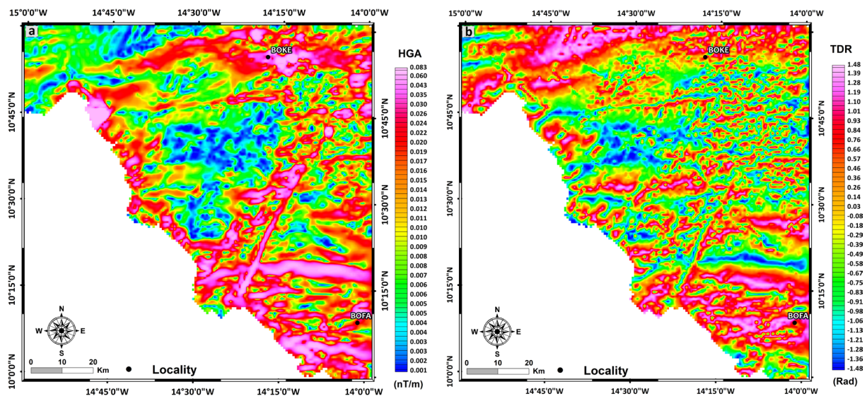
Figure 6. Horizontal gradient amplitude (a) and tilt derivative (b) of the RTE field.
