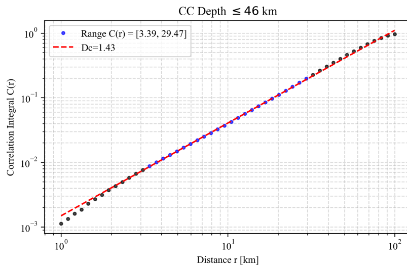
Figure F8. Fractal dimension ( D_c ) estimation for seismic events shallower than 46 km in the Campo Colorado.
