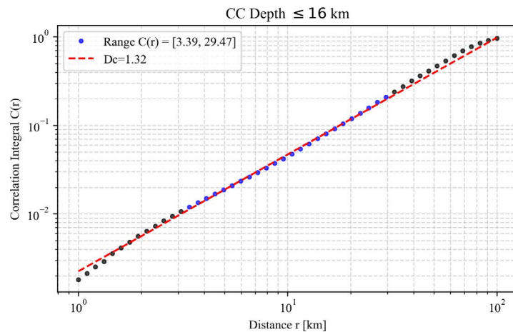
Figure F3. Fractal dimension ( D_c ) estimation for seismic events shallower than 16 km in the Campo Colorado.
