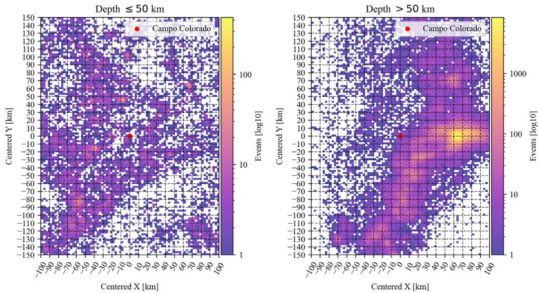
Figure B4. Zoomed view of the area of interest centered on the coordinates of Campo Colorado. Separate density maps are shown for cortical events ( \leq 50 km) and deep events ( > 50 km).
