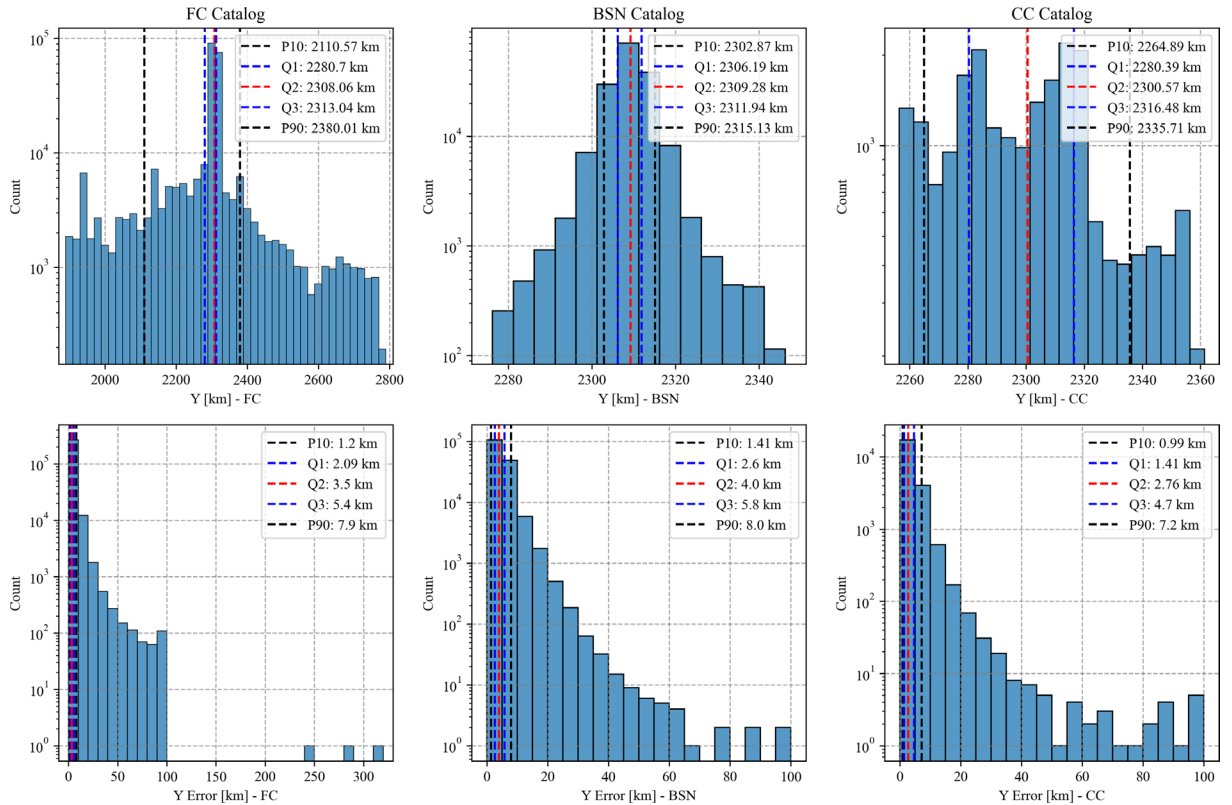
Figure C2. Histograms of the Y-coordinate location and corresponding location uncertainties for seismic events in the three analyzed subcatalogs.
