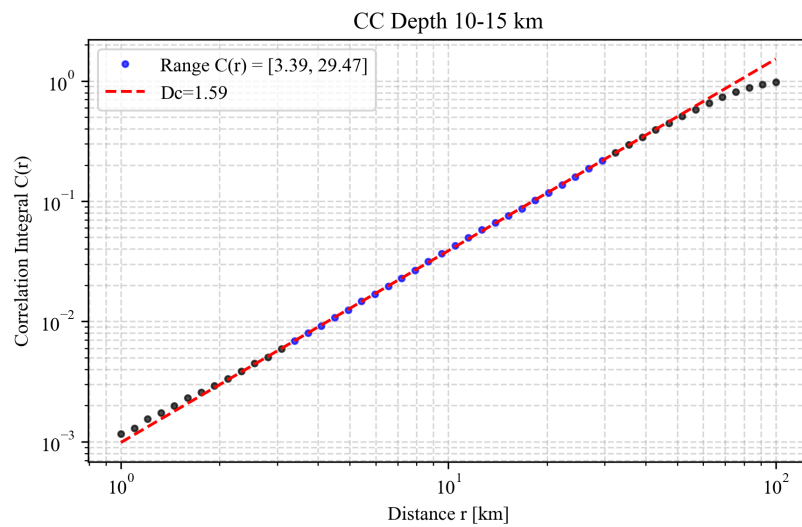
Figure F12. Estimated fractal dimension ( D_c ) for seismic events within the 10-15 km depth interval in the Campo Colorado.
