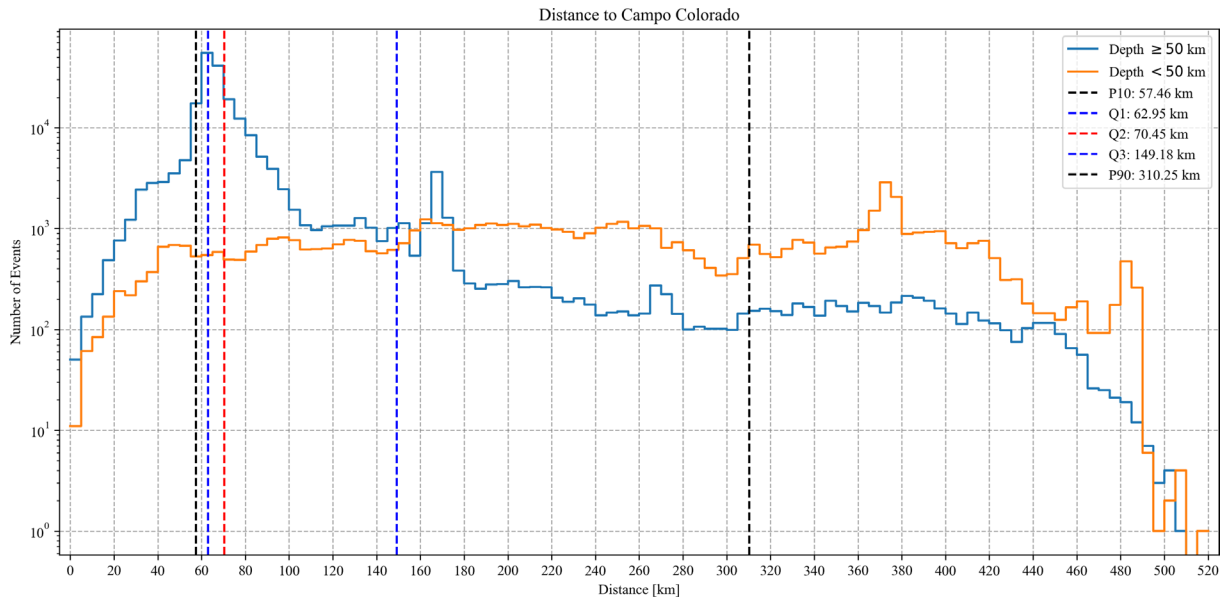
Figure 5. Histogram of the planar (XY) distance of seismic events relative to Campo Colorado. Crustal events ( \leq 50 km depth, orange) and deep events ( > 50 km depth, blue) are shown separately. A marked increase in the number of deep events is observed at a distance of approximately 60 km, corresponding to the location of the Bucaramanga Seismic Nest. In contrast, crustal events are sparse near Campo Colorado and increase progressively with distance.
