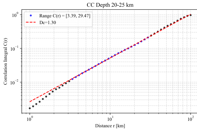
Figure F13. Estimated fractal dimension ( D_c ) for seismic events within the 20-25 km depth interval in the Campo Colorado.
