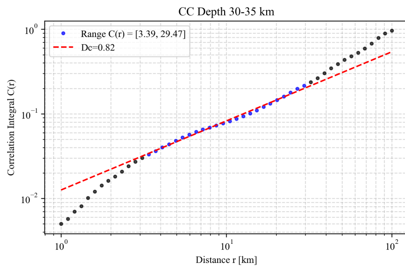
Figure F14. Estimated fractal dimension ( D_c ) for seismic events within the 30-35 km depth interval in the Campo Colorado.
