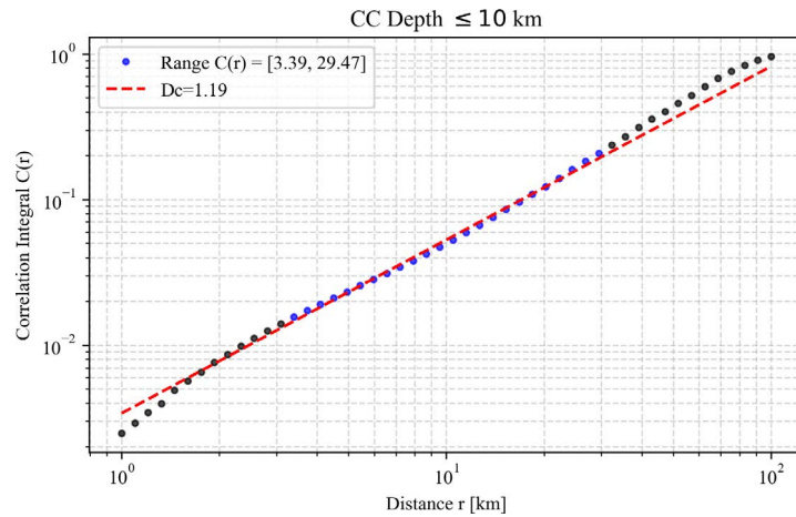
Figure F2. Fractal dimension ( D_c ) estimation for seismic events shallower than 10 km in the Campo Colorado.
