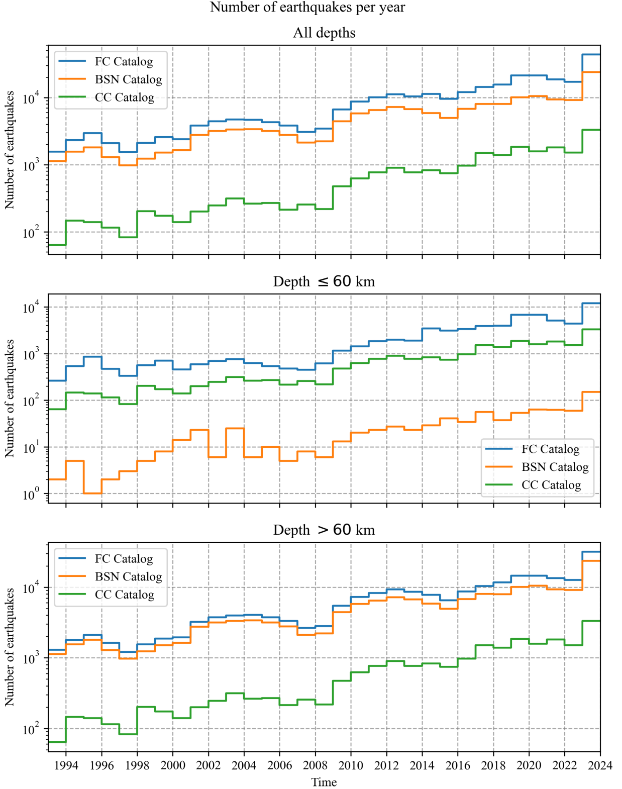
Figure 7. Yearly seismicity rates for the three subcatalogs, shown for the complete dataset, crustal events ( \leq 60 km), and deep events ( > 60 km).
