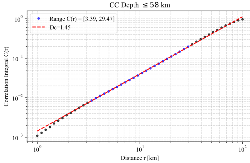
Figure F10. Fractal dimension ( D_c ) estimation for seismic events shallower than 58 km in the Campo Colorado.
