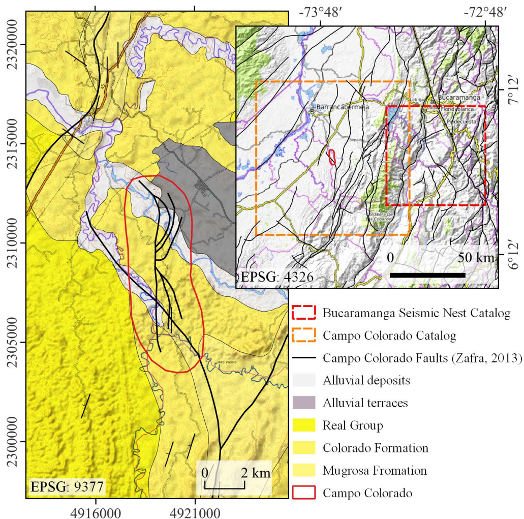
Figure 2. Location of Campo Colorado within the Campo Colorado Catalog (CC) area and geological characterization of the sector considered for potential CO 2 injection. The area exhibits a well-developed fault system and is mainly composed of clastic sedimentary rocks.
