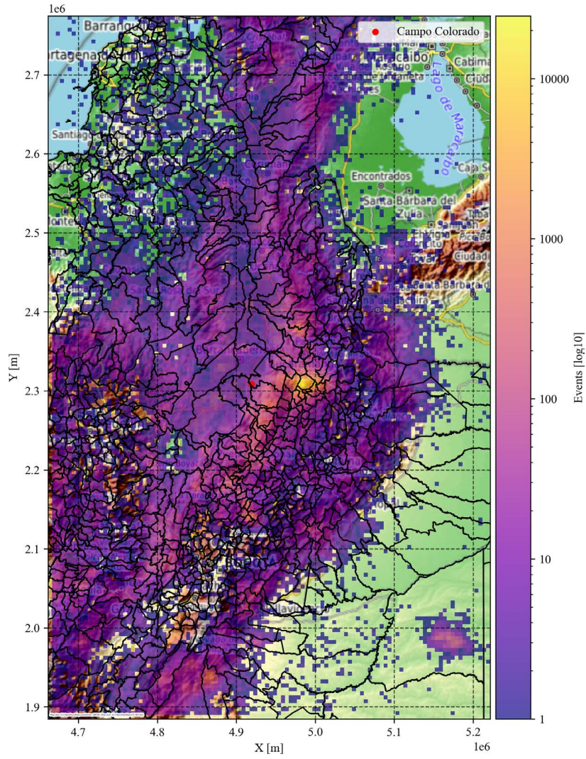
Figure B3. Heatmap showing the spatial distribution of events from the unified catalog. The red point marks the location of Campo Colorado. The highest event concentration coincides with the Bucaramanga Seismic Nest.
