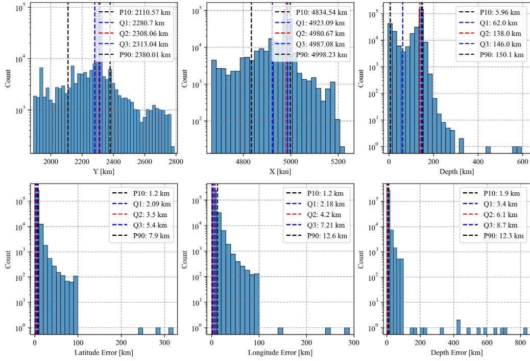
Figure B1. Histograms showing the distribution of event location coordinates and their corresponding location uncertainties.
