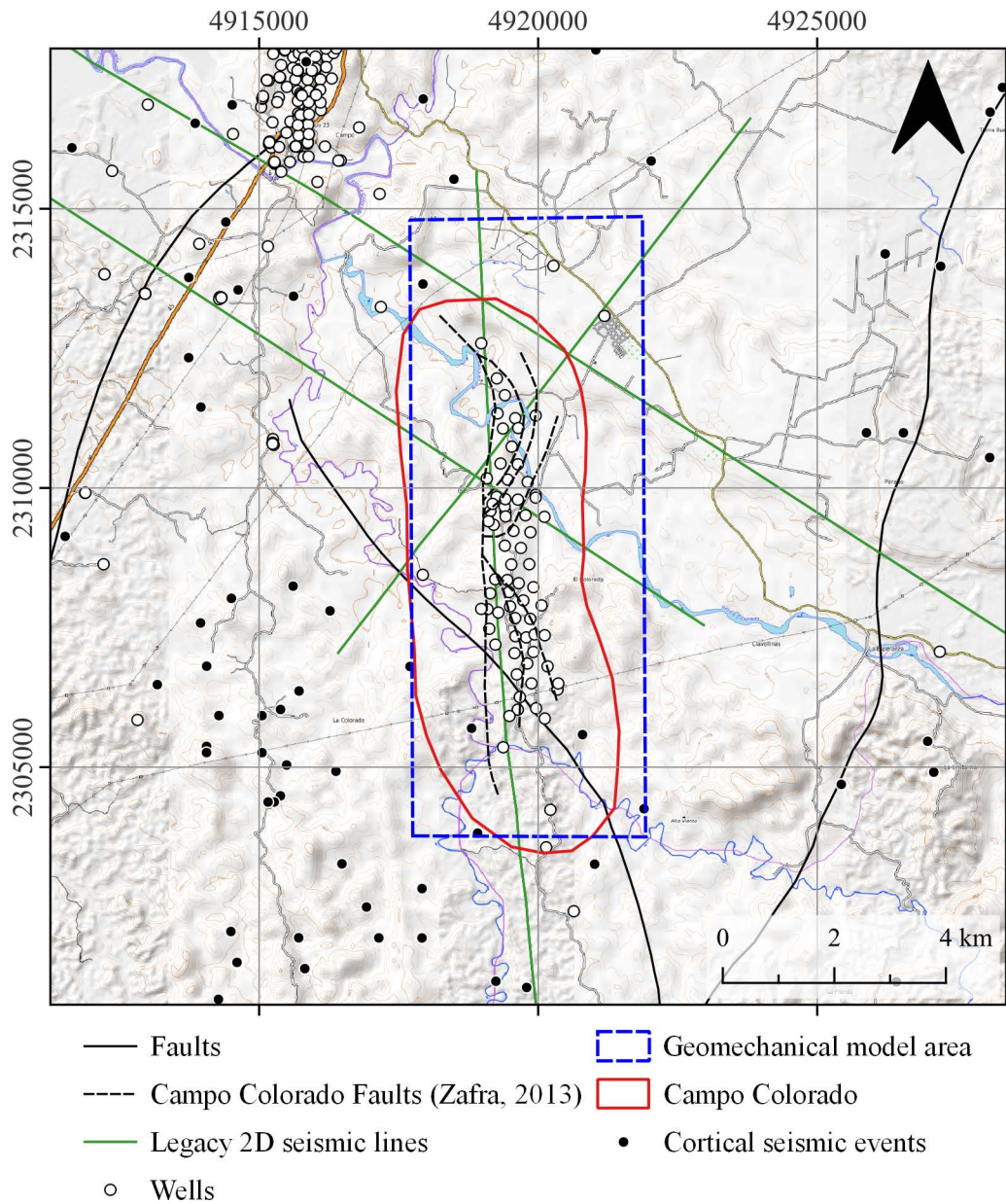
Figure 18. Location of the proposed CO 2 storage site at Campo Colorado showing the geomechanical modeling domain, existing wells, interpreted faults, legacy 2D seismic lines, and the distribution of crustal seismicity.
