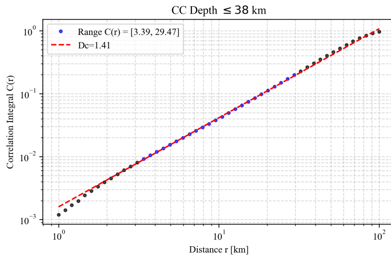
Figure F7. Fractal dimension ( D_c ) estimation for seismic events shallower than 38 km in the Campo Colorado.
