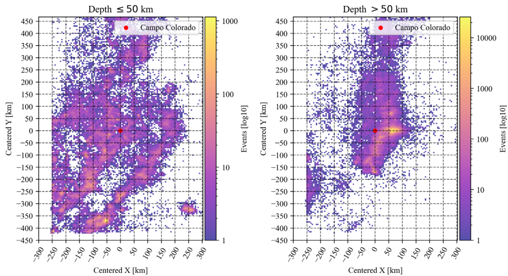
Figure 4. Heat maps of the spatial distribution of seismic events from the unified catalog, centered relative to Campo Colorado (red point). Separate heat maps are shown for crustal events ( \leq 50 km) and deep events ( > 50 km), highlighting a greater concentration of deep seismicity compared to crustal events. This pattern reflects the dominance of seismic activity associated with the Bucaramanga Seismic Nest, located approximately 50 km east (X direction) of Campo Colorado.
