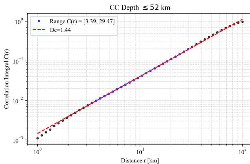
Figure F9. Fractal dimension ( D_c ) estimation for seismic events shallower than 52 km in the Campo Colorado.
