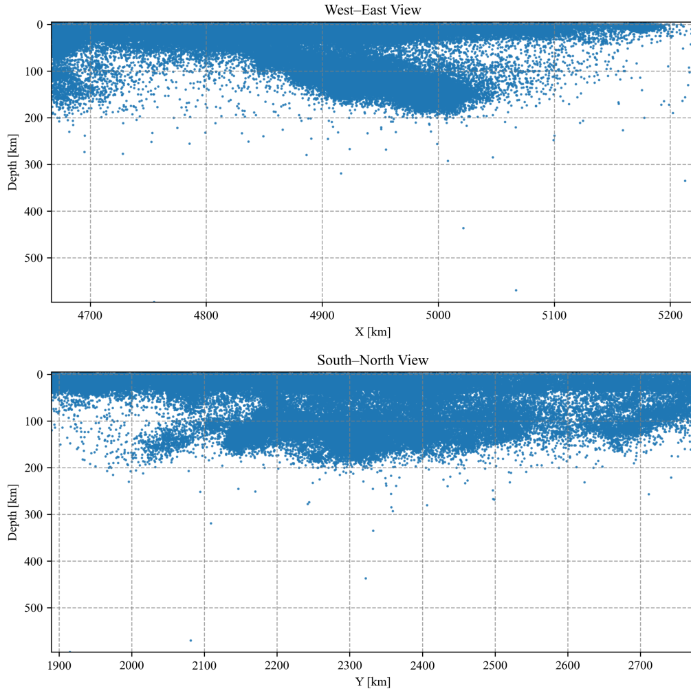
Figure 3. Cross-sections generated from the X and Y projections of the events in the unified catalog.
