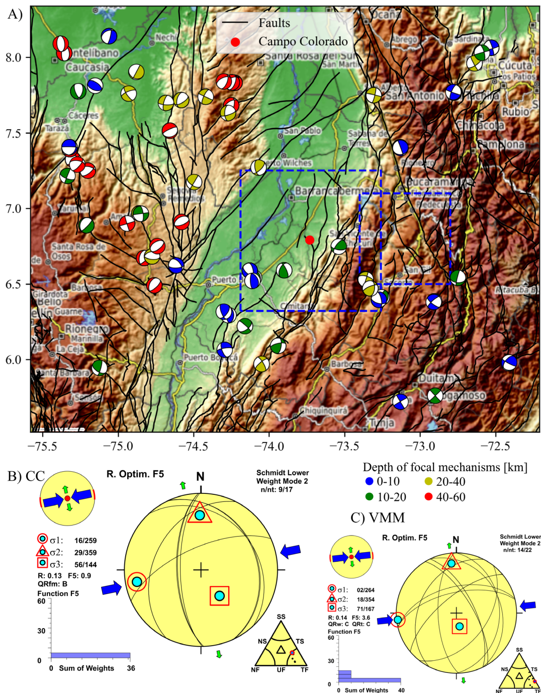
Figure 16. A) Focal mechanisms compiled from the SGC, ISC, and CMT catalogs for the regional study area. Based on this information, a stress inversion analysis was performed using the WinTensor software to estimate the stress field distribution. B) Stress inversion results for the Campo Colorado (CC) area. C) Stress inversion results for the Middle Magdalena Valley (VMM).
