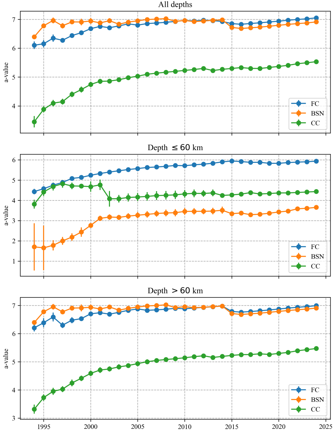
Figure 9. Temporal evolution of the cumulative a-value for the three subcatalogs, calculated by progressively extending the catalog year by year, for all events, crustal events ( \leq 60 km), and deep events ( > 60 km). Vertical bars indicate the standard deviation obtained through resampling.
