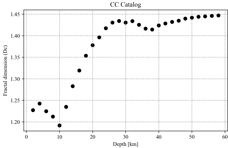
Figure 14. Fractal dimension ( D_c ) values calculated for cortical seismic events in the CC area, estimated incrementally as a function of depth.
