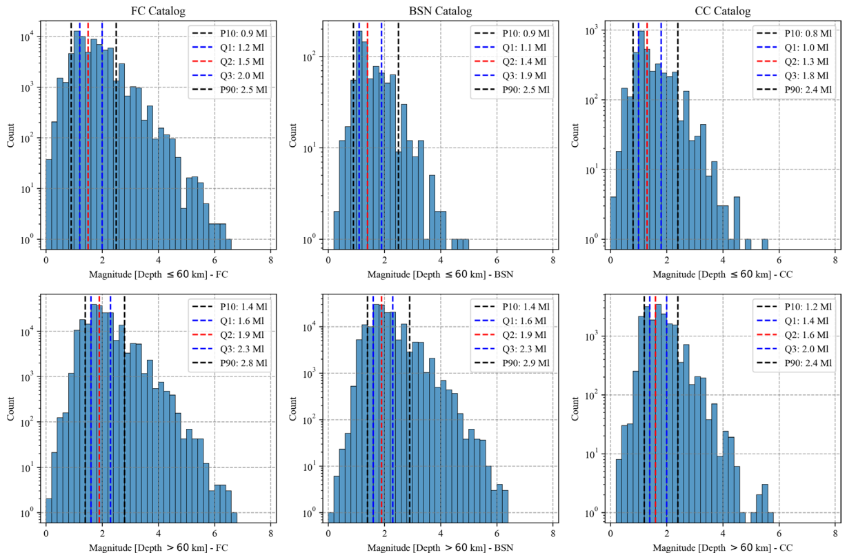
Figure 6. Magnitude histograms for the three subcatalogs, separated into crustal events ( \leq 60 km depth) and deep events ( > 60 km depth).
