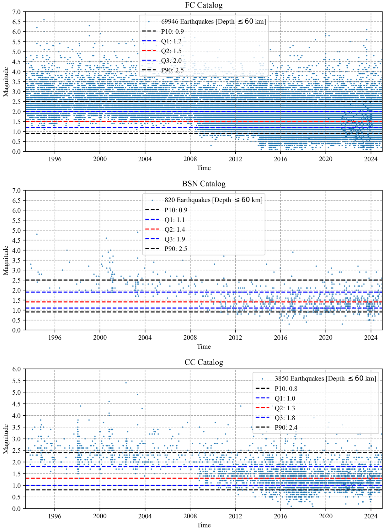
Figure C4. Time-magnitude plots of seismic events from the three subcatalogs, considering only cortical events ( \leq 60 km).
