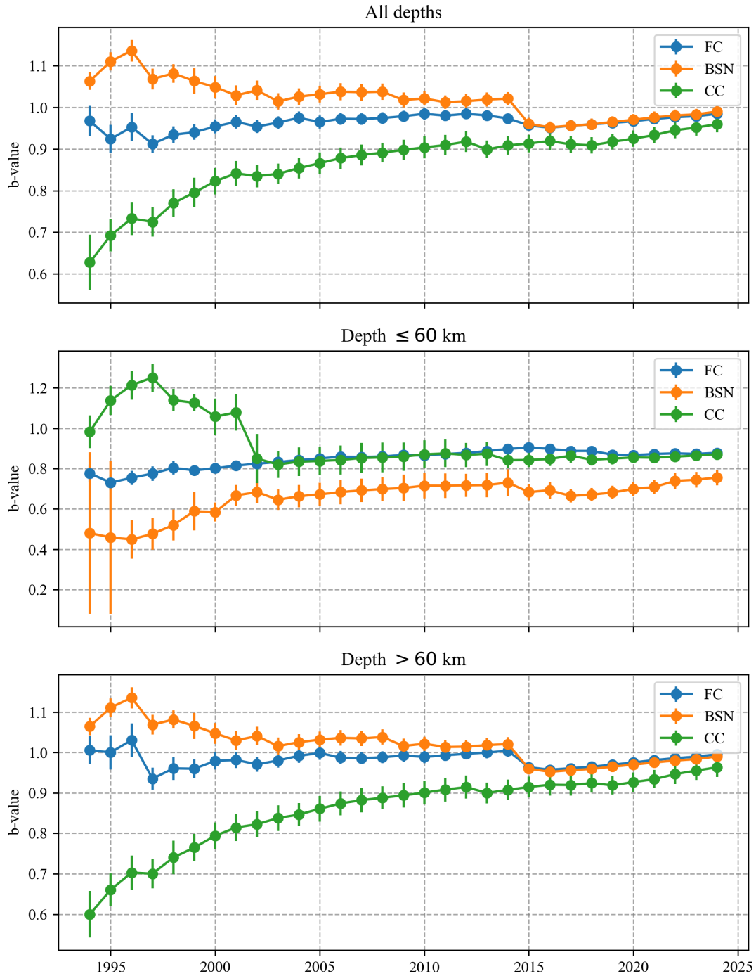
Figure 10. Temporal evolution of the cumulative b -value for the three subcatalogs, calculated by progressively extending the catalog year by year, for the complete dataset, crustal events ( \leq 60 km), and deep events ( > 60 km). Vertical bars indicate the standard deviation obtained through resampling.
