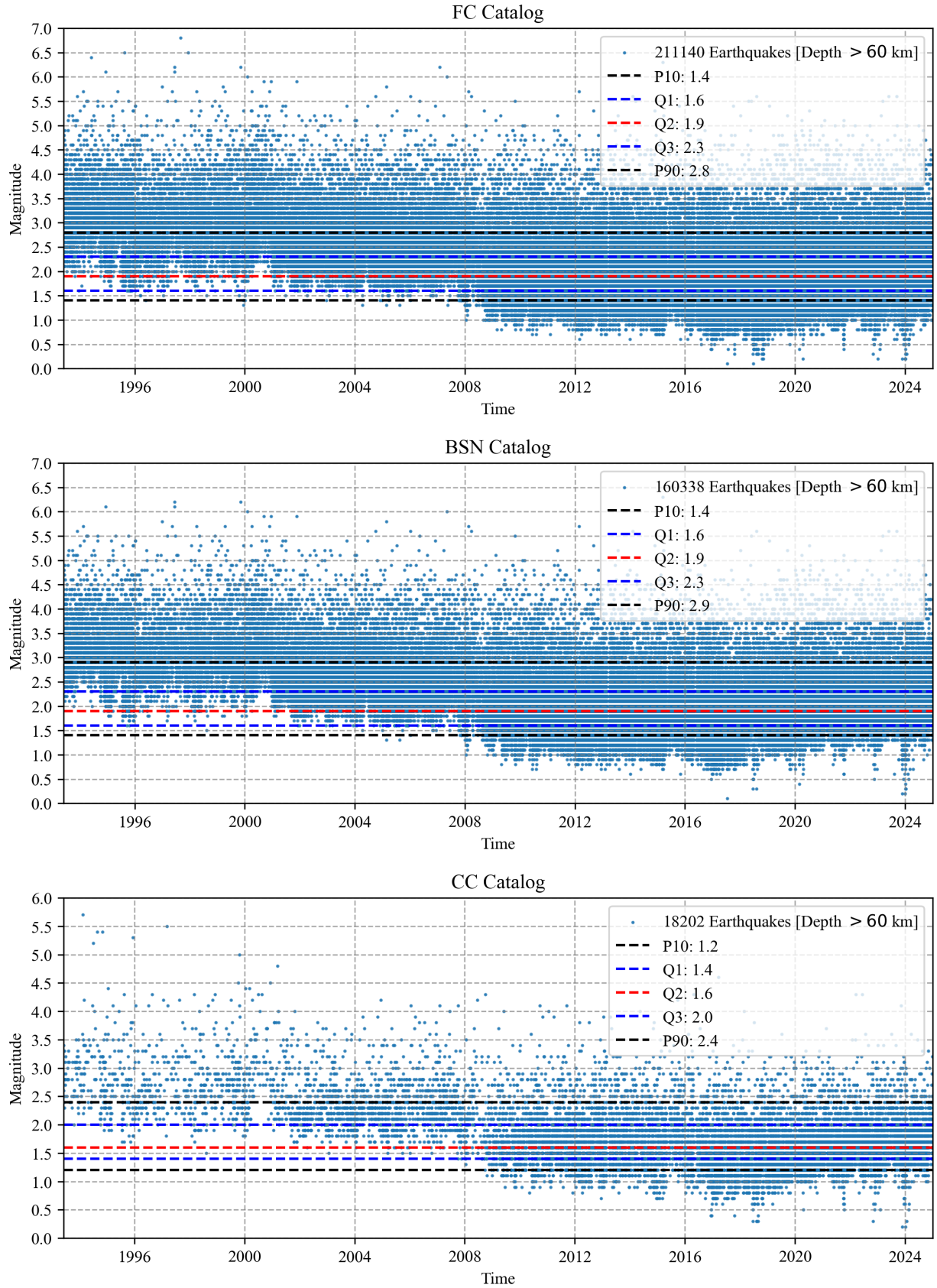
Figure C5. Time-magnitude distribution of deep seismic events (>60 km) for the three analyzed subcatalogs.
