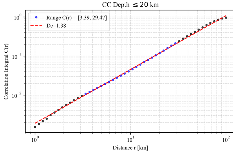
Figure F4. Fractal dimension ( D_c ) estimation for seismic events shallower than 20 km in the Campo Colorado.
