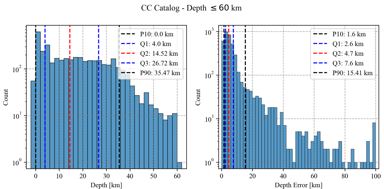
Figure 13. Frequency distribution of seismic event depths and their corresponding depth location errors in the Campo Colorado area.
