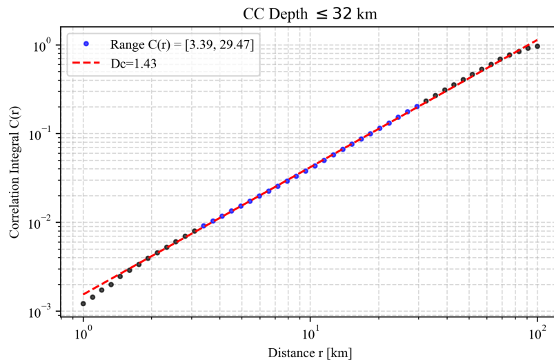
Figure F6. Fractal dimension ( D_c ) estimation for seismic events shallower than 32 km in the Campo Colorado.
