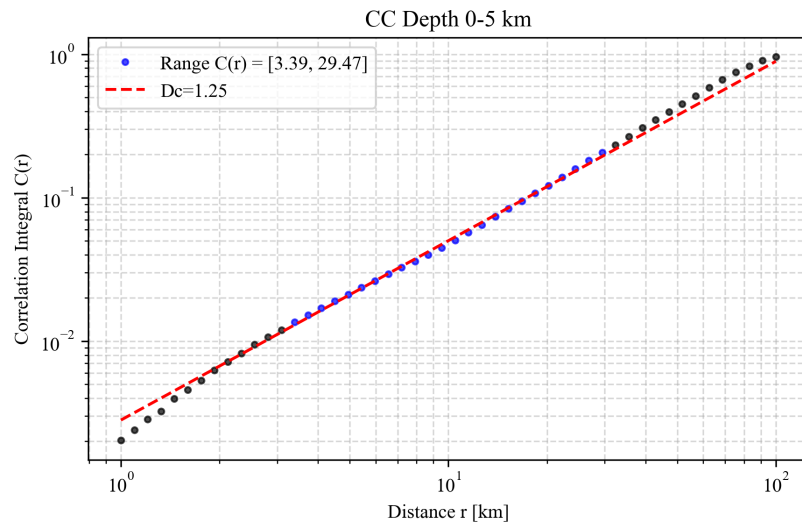
Figure F11. Estimated fractal dimension ( D_c ) for seismic events within the 0-5 km depth interval in the Campo Colorado.
