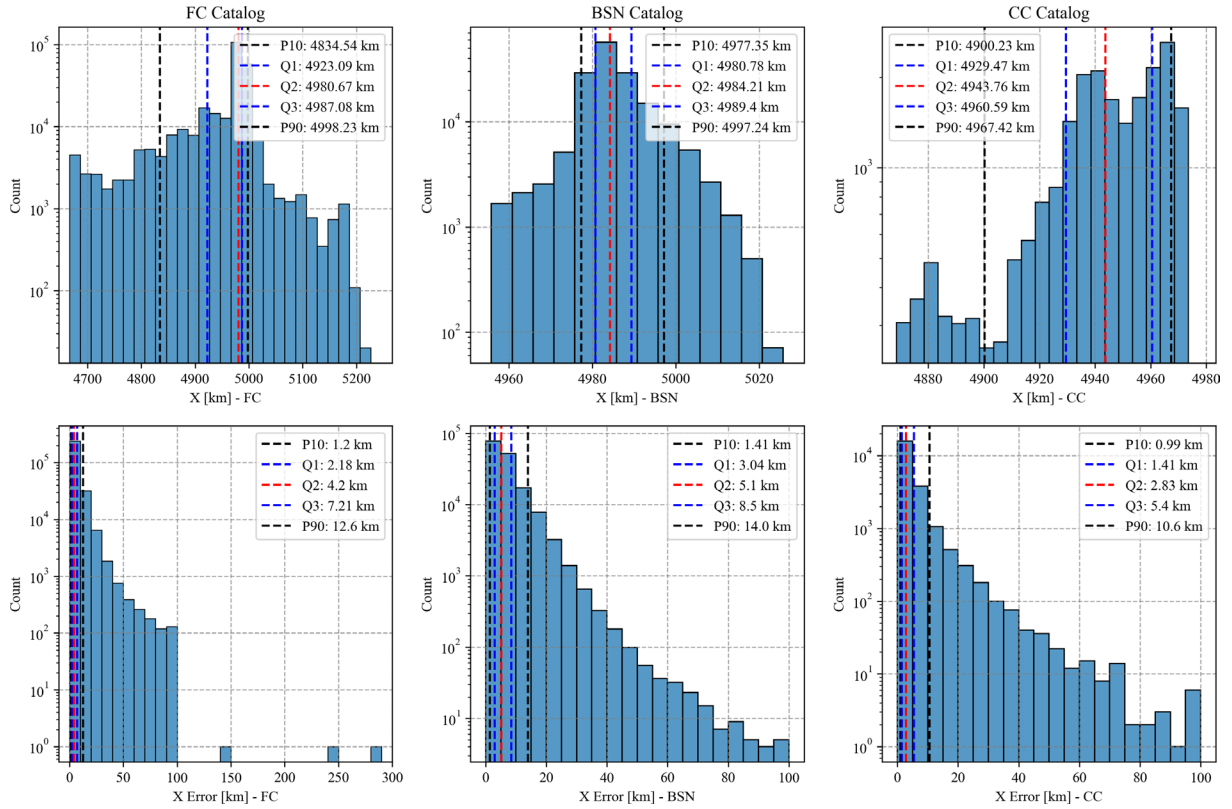
Figure C1. Histograms of the X-coordinate location and corresponding location uncertainties for seismic events in the three analyzed subcatalogs.
