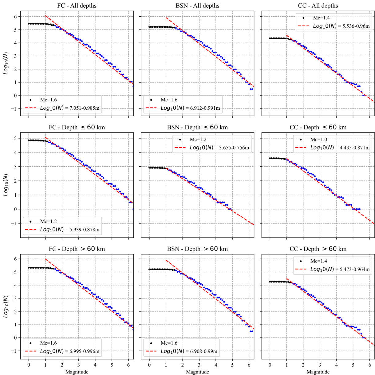
Figure 8. Estimated Gutenberg-Richter parameters (a-value, b-value, and M_c ) for the three subcatalogs, computed for the complete dataset, crustal events ( \leq 60 km), and deep events ( > 60 km).
