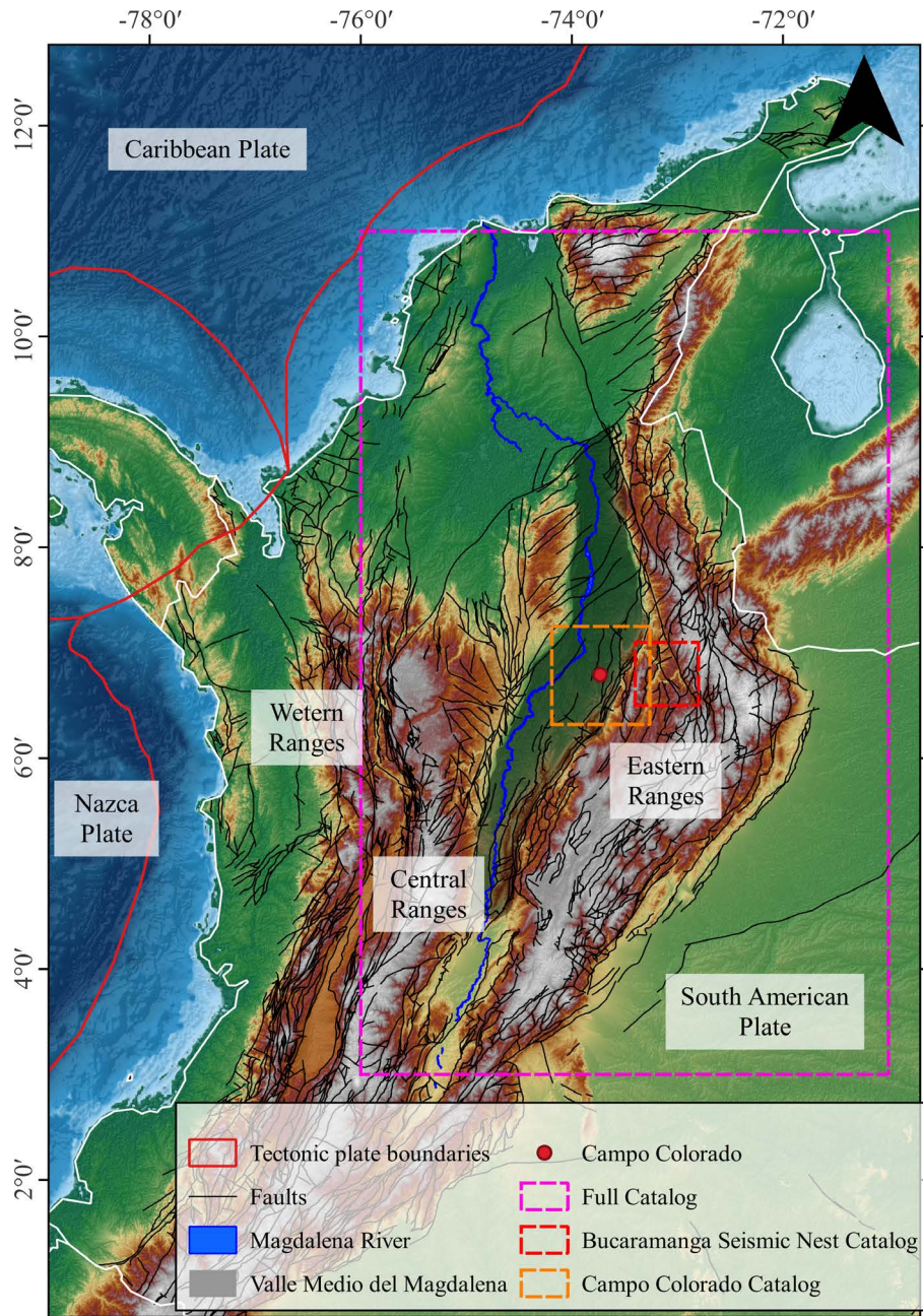
Figure 1. Location map of the study area and the spatial extent of the three seismic subcatalogs analyzed in Colombia: the Full Catalog (FC), the Bucaramanga Seismic Nest Catalog (BSN), and the Campo Colorado Catalog (CC). The FC represents the complete dataset used for regional-scale analysis. The BSN is restricted to events associated with the Bucaramanga Seismic Nest, recognized as the most seismically active zone in Colombia. The CC corresponds to the local study area, focusing on seismicity in the vicinity of the Campo Colorado field.
