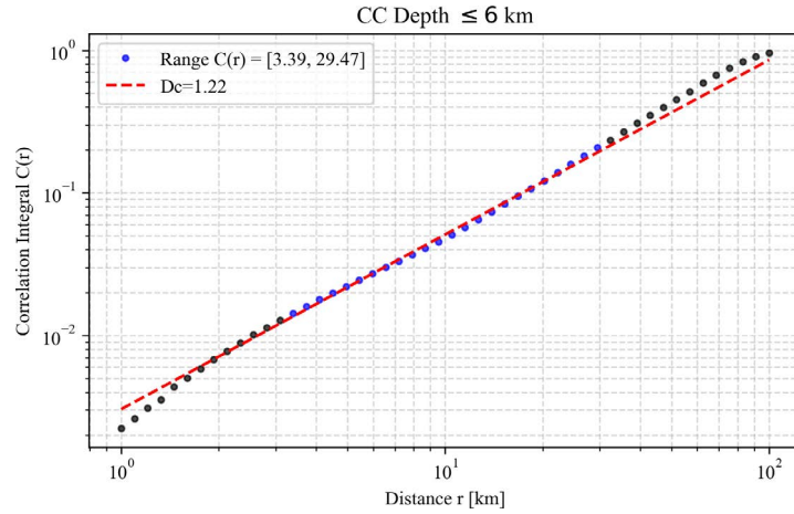
Figure F1. Fractal dimension ( D_c ) estimation for seismic events shallower than 6 km in the Campo Colorado.
