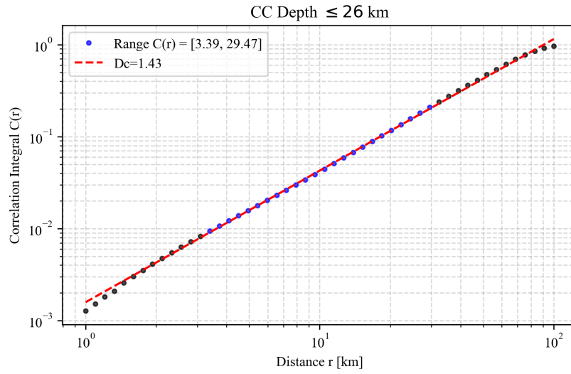
Figure F5. Fractal dimension ( D_c ) estimation for seismic events shallower than 26 km in the Campo Colorado.
