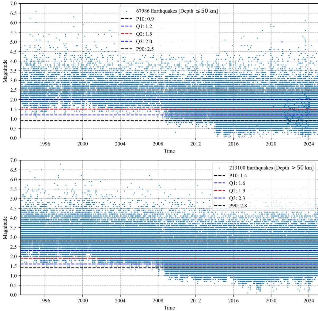
Figure B2. Time-magnitude plot of the unified catalog, differentiating events up to a depth of 50 km, considering that the TECTO and LBG catalogs only include events within this depth range.
