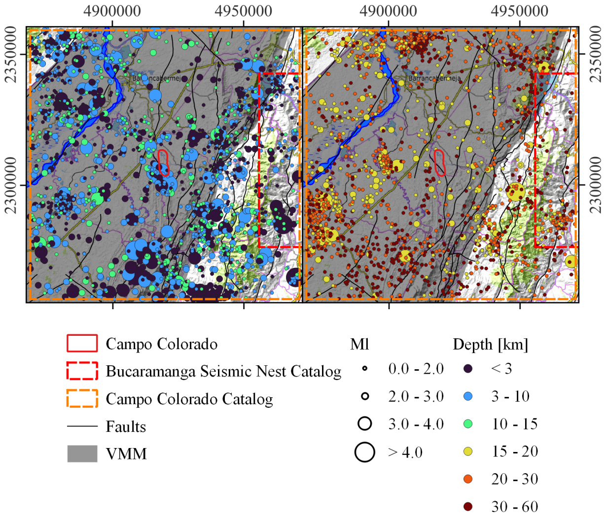
Figure 17. Spatial distribution of cortical seismic events associated with the CC within a 100 \times 100 km polygon centered on the study area. Shallower events are displayed in cool colors, whereas deeper events are represented in warm colors.
