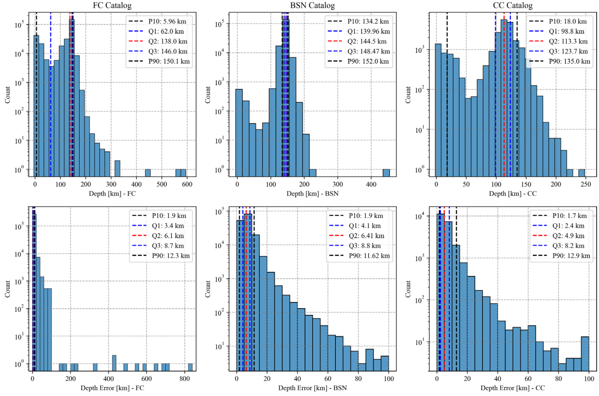
Figure C3. Histograms of the Depth location and corresponding location uncertainties for seismic events in the three analyzed subcatalogs.
