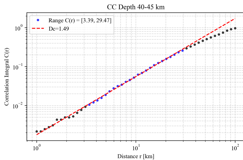
Figure F15. Estimated fractal dimension ( D_c ) for seismic events within the 40-45 km depth interval in the Campo Colorado.
