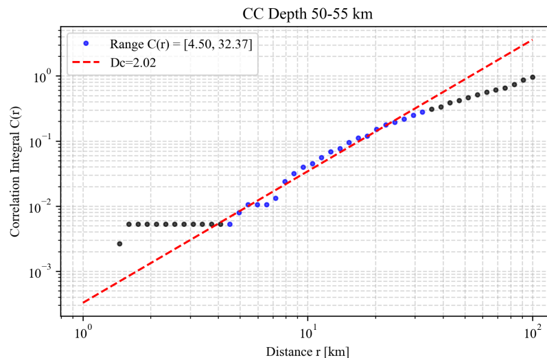
Figure F16. Estimated fractal dimension ( D_c ) for seismic events within the 50-55 km depth interval in the Campo Colorado.
