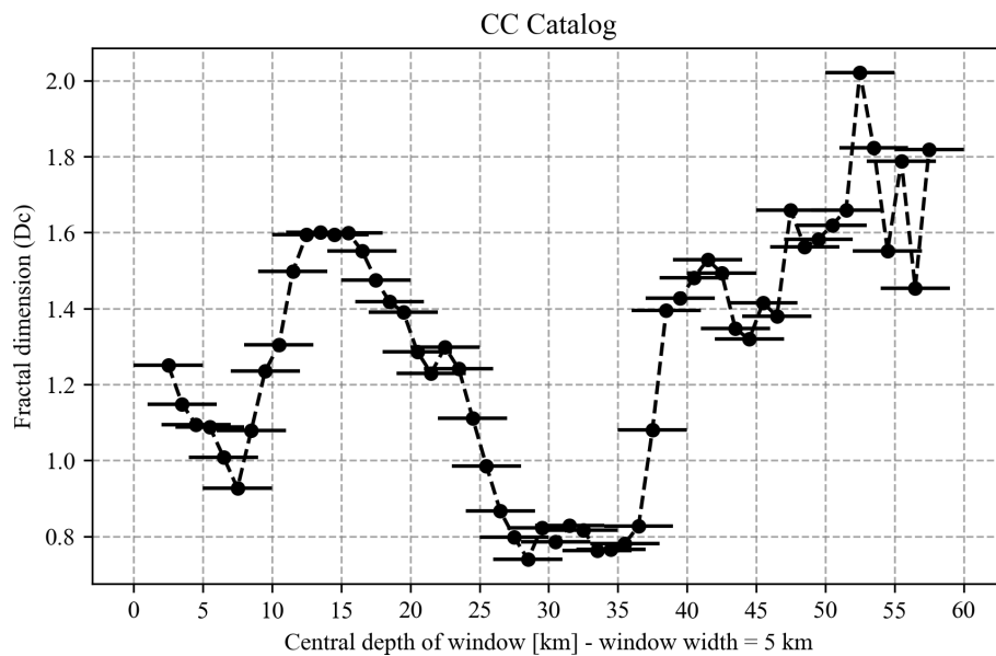
Figure 15. Fractal dimension ( D_c ) calculated for cortical seismic events in the CC area using a moving depth window. Points along the X-axis represent the center of each depth window, while the associated horizontal bars indicate the window width (5 km).
